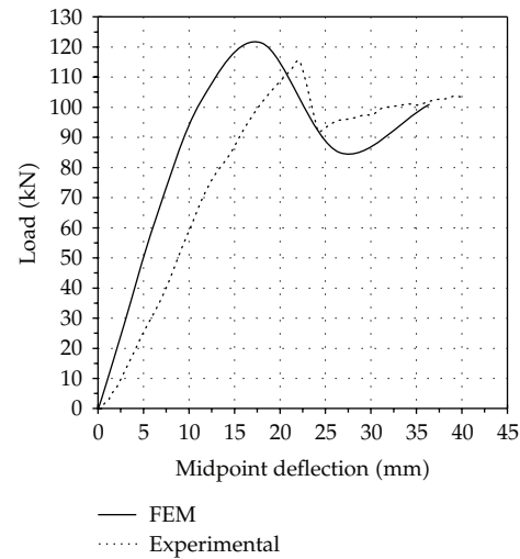
(c) Comparison of numerical and experimental test results
