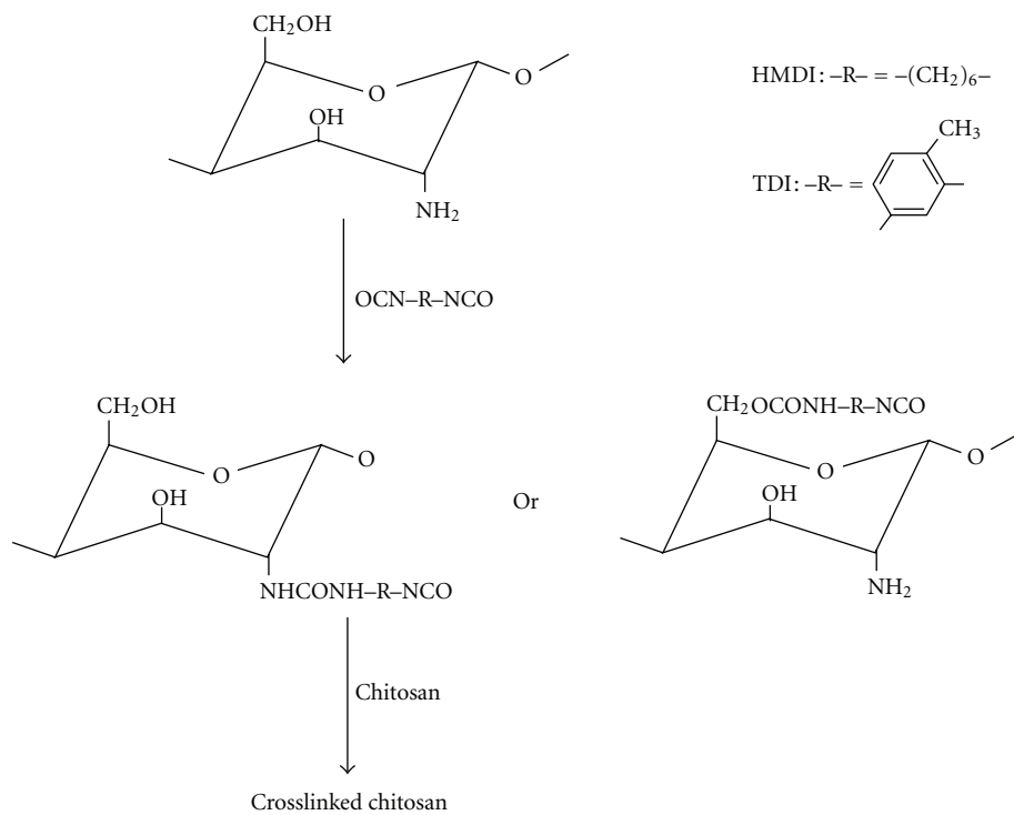
SCHEME 1: Crosslinking by diisocyanate.
