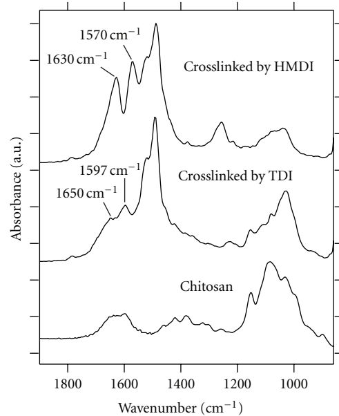
FIGURE 3: Infrared spectra for the hollow chitosan capsules crosslinked by HMDI and TDI, and for original chitosan (as a reference). The positions on the vertical axis are shifted to enable the profiles to be distinguished.
