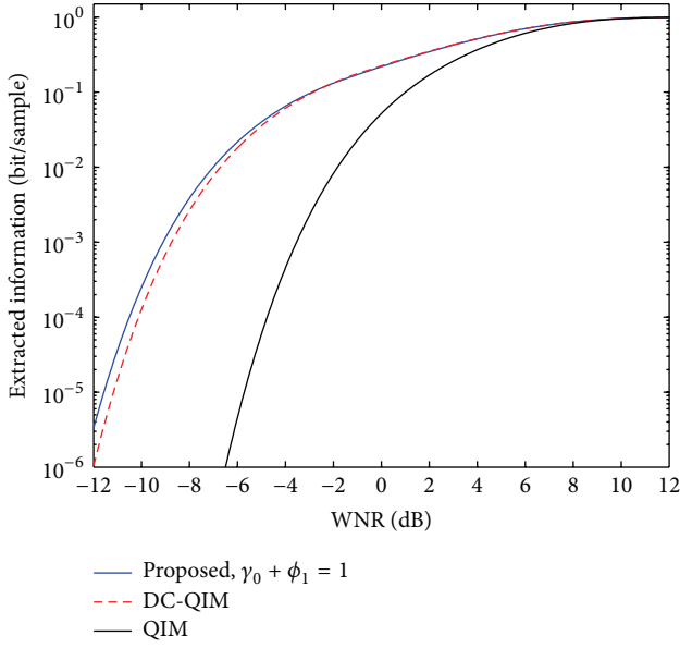
FIGURE 6: Analytic-based estimation of information extracted under AWGN without IDL.
