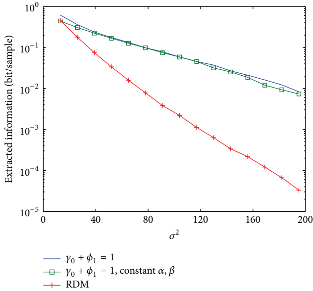
FIGURE 9: Information extracted under GA followed by AWGN.
