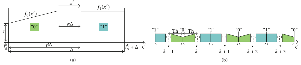
FIGURE 1: Distribution of the quantized coefficients: (a) Inside k th embedding interval. (b) In five consecutive intervals.
