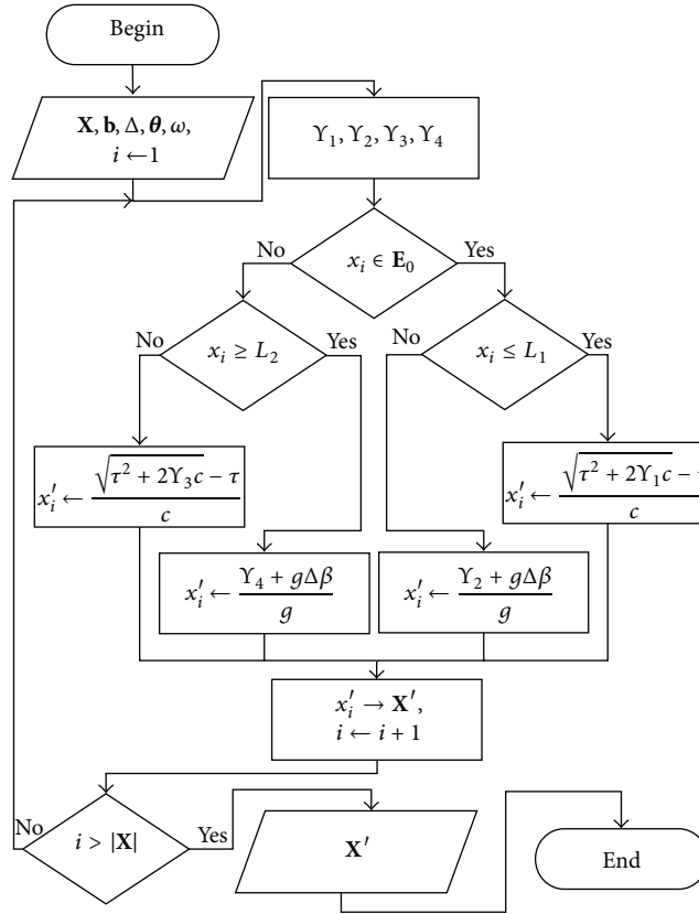
FIGURE 5: Quantization diagram for the k th embedding interval.
