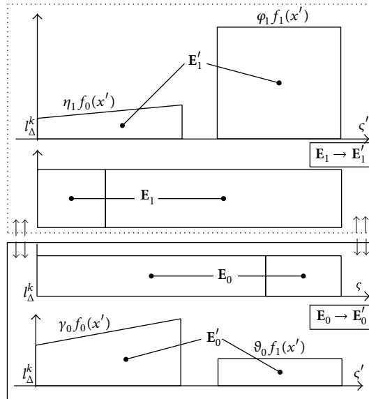
FIGURE 4: Scheme of redistribution of original samples during quantization, \Omega is “false.”
