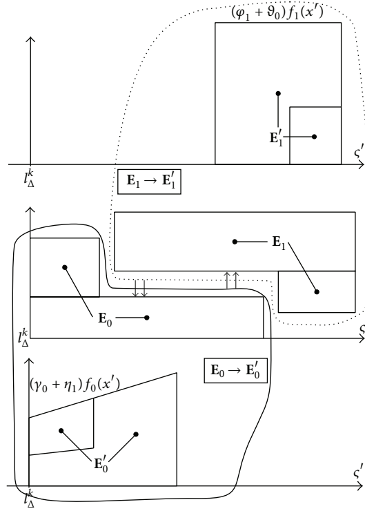
FIGURE 3: Scheme of redistribution of original samples during quantization, \Omega is “true.”
