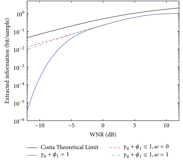
FIGURE 7: Analytic-based estimation of information extracted under AWGN with IDL.
