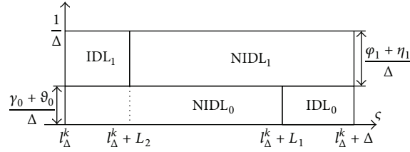
FIGURE 2: Scheme of labeling and distribution of original samples prior to quantization.
