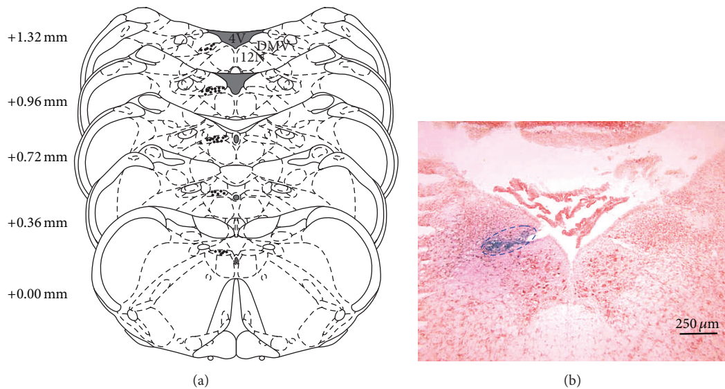
FIGURE 1: Histological sites of micropipette tips in the DMV of the rat. Reconstruction detailing microinjection sites of chemical into the DMV in the brain atlas, with the dots indicating the micropipette tips. Numbers indicate distance from the obex in the anteroposterior plane. 4V: the 4th ventricle, 12N: the hypoglossal nucleus (a). Representative brain stem section showing the position of DMV, with ellipse and blue macula indicating DMV (b).
