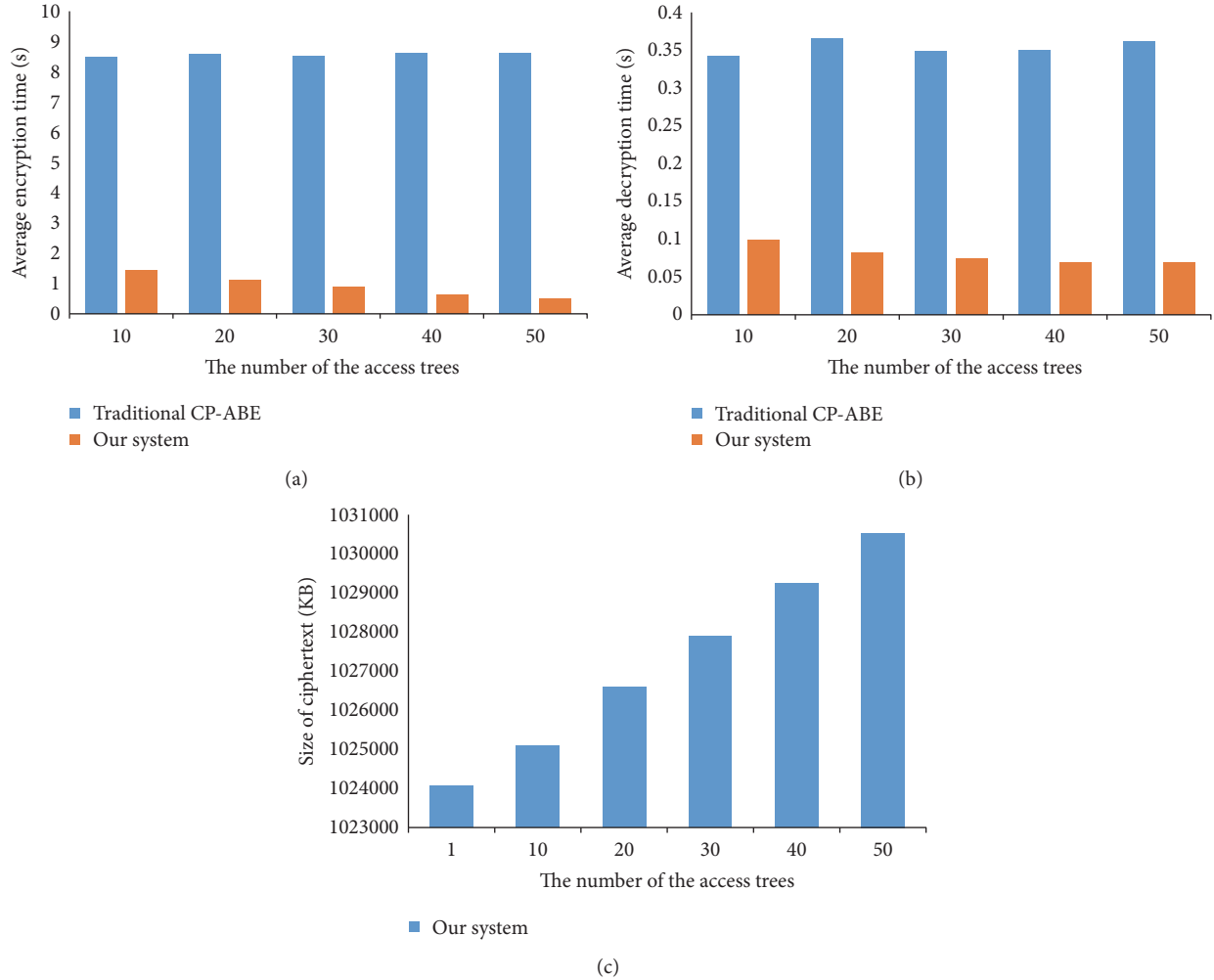
FIGURE 5: (a) Comparison of the average encryption times between CPABE and our system, when the number of access trees is different. (b) Comparison of decryption times between CPABE and our system, when the number of access trees is different. (c) Changes in the ciphertext size of our system, when the number of access trees is different.
