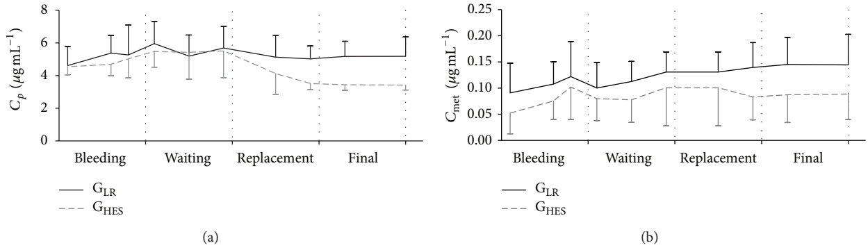
FIGURE 1: Propofol plasma concentration ( C_p — \mu\text{g/mL} ) and propofol free metabolites ( C_{met} — \mu\text{g/mL} ) during the four phases of the study. The two groups are shown: G_{LR} —black line and G_{HES} —dashed grey line.
