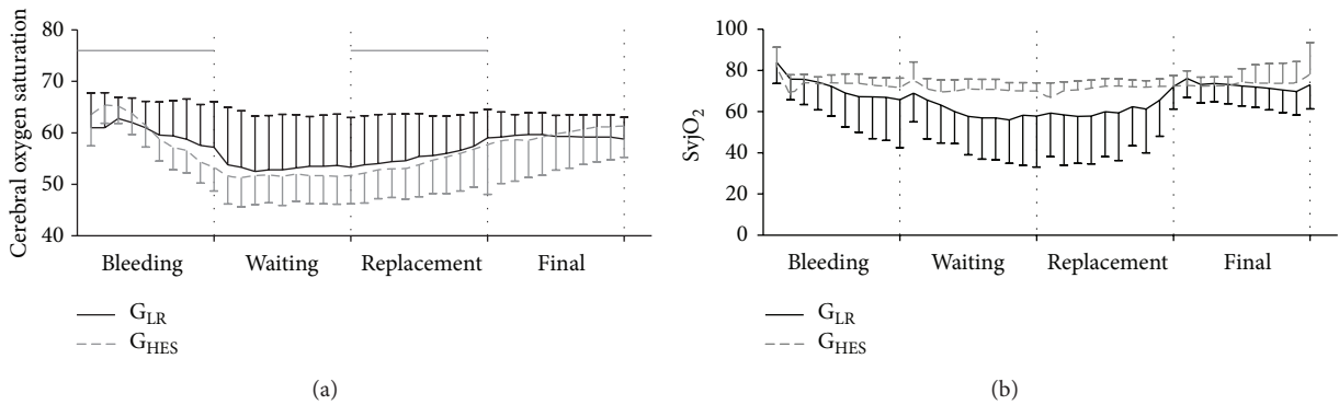
FIGURE 2: Cerebral oxygenation parameters during the four phases of the study: cerebral oxygen saturation (INVOS) (a) and Sv_jO_2 (%) (b). The two groups are shown: G_{LR} —black line and G_{HES} —dashed grey line.
