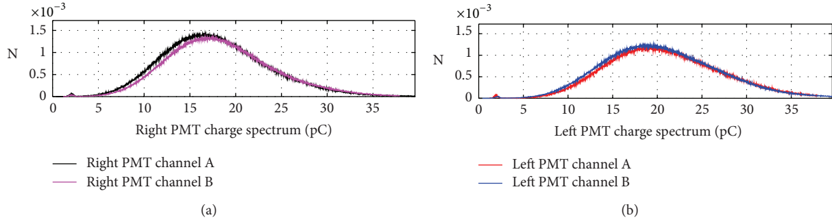
FIGURE 6: Charge spectra for the Right PMT (a) and for the Left PMT (b) obtained by injecting the UV laser into the center of the fiber ribbon and reversing the electronic chains.
