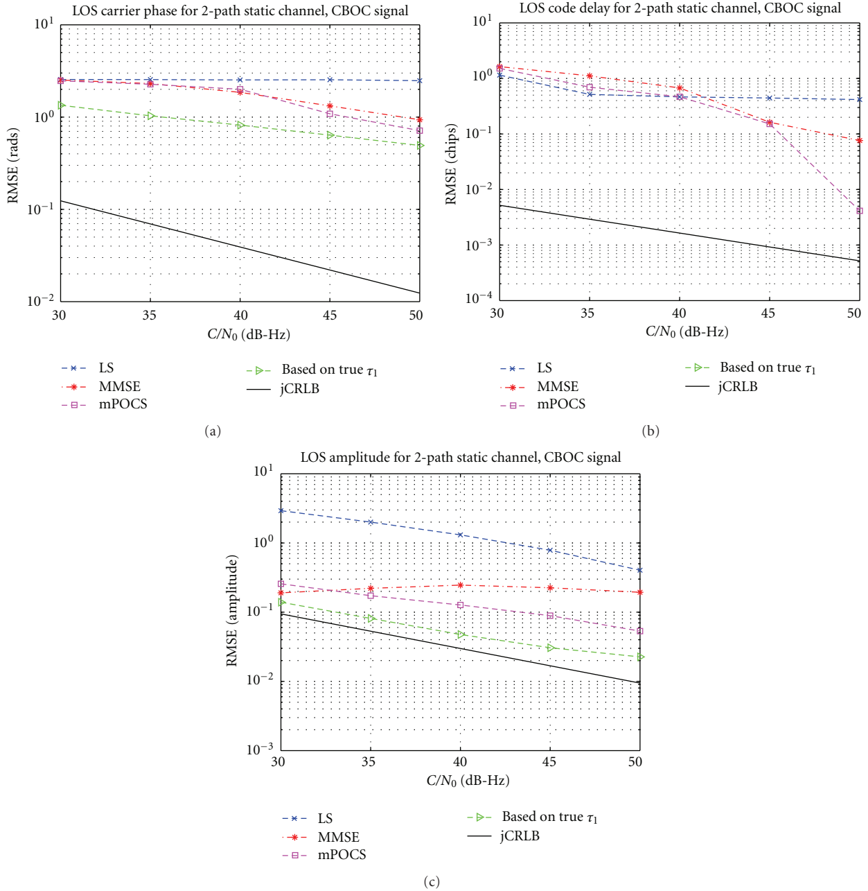
FIGURE 5: LOS carrier phase (a), code delay (b), and amplitude (c) versus C/N_0 for 2-path static channel and CBOC signal.
