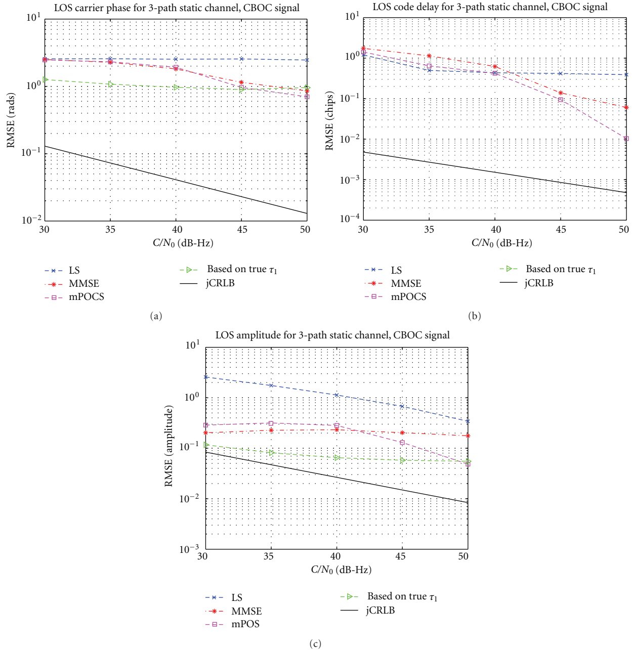
FIGURE 7: LOS carrier phase (a), code delay (b), and amplitude (c) versus C/N_0 for 3-path static channel and CBOC signal and N_c = 2 .
