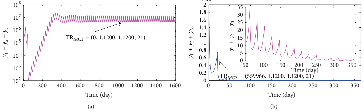
FIGURE 7: (a) and (b) present the variances of the number of tumor cells when taking the combination chemotherapy regimens TR_{MC1} and TR_{MC2} , respectively.
