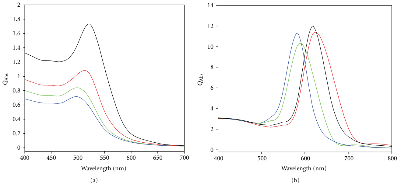
FIGURE 6: Comparison between the absorption spectra at (a) \theta = 0^\circ and (b) \theta = 90^\circ for a nanobar (black line), a plain cylinder (red line), an ellipsoid (blue line), and a capped spherical cylinder (green line).
