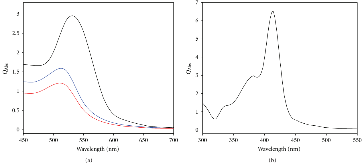
FIGURE 3: The calculated absorption spectrum for (a) a gold nanocube of width 50 nm (black), a sphere of diameter 50 nm (red), and a sphere that has the same volume as the nanocube (blue), (b) a silver nanocube of width 50 nm.
