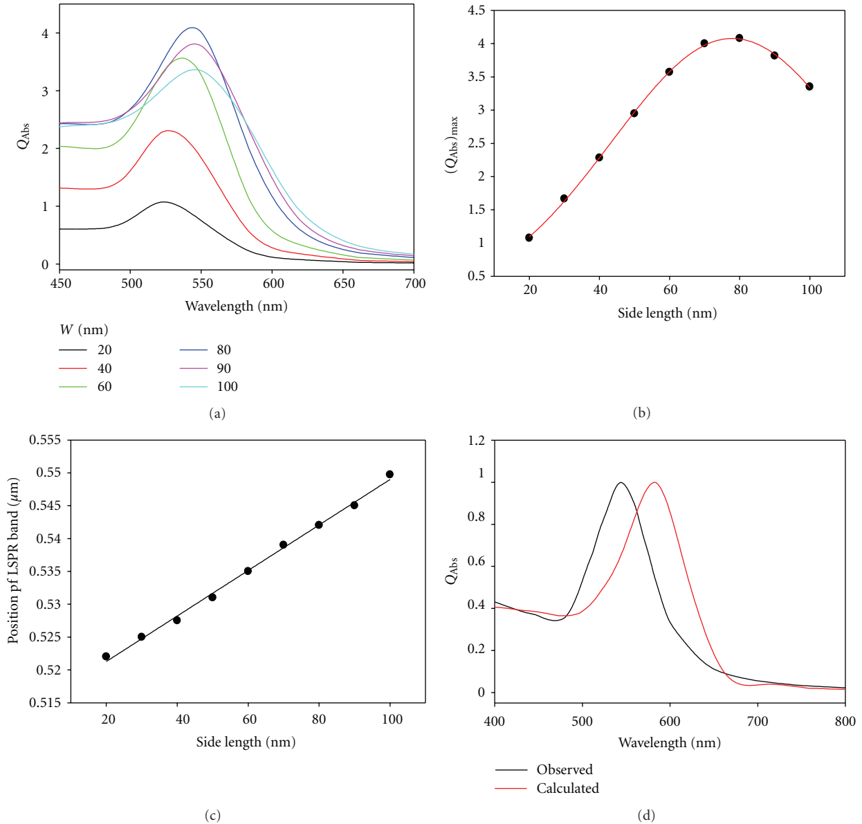
FIGURE 2: (a) Dependency of the absorption spectrum on the nanocube width, (b) the maximum absorption efficiency as a function of the width, (c) position of the LSPR band versus the nanocube width, and (d) comparison between observed and calculated absorption spectra of a gold nanocube of width 45 nm.
