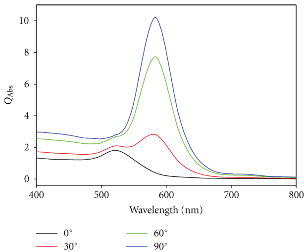
FIGURE 4: Absorption spectra for a gold nanobar (40 × 80 nm) at different incident angles and p-polarized light.
