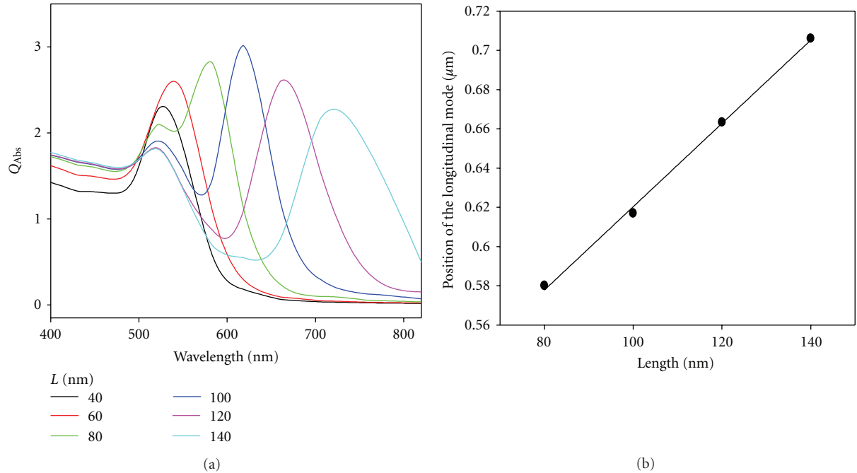
FIGURE 5: (a) Calculated absorption spectra of a nanobar of width of 40 nm and different aspect ratios at \theta = 30^\circ , (b) position of the longitudinal band versus the nanobar length.
