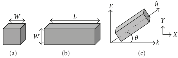
FIGURE 1: Structural parameters of (a) a cube, (b) a nanobar, (c) orientation of the nanobar with respect to the incident radiation (p-polarized light).
