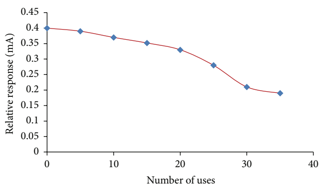
FIGURE 13: Reusability of the present method.
