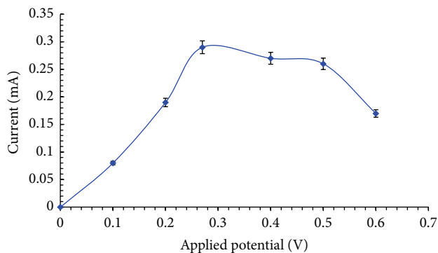
FIGURE 6: Response of current with applied potential.
