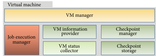
FIGURE 3: The structure of virtual machine.
