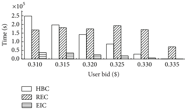
FIGURE 14: Comparison of rollback time according to user bid.
