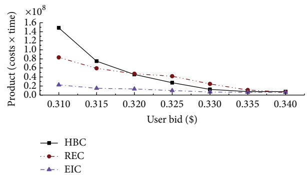
FIGURE 17: Comparison of combined metrics (total task execution time and costs).
