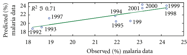
FIGURE 6: Correlation between independently predicted and observed number of malaria cases (% of malaria cases from the total number of people who come to the regional hospitals with fever).
