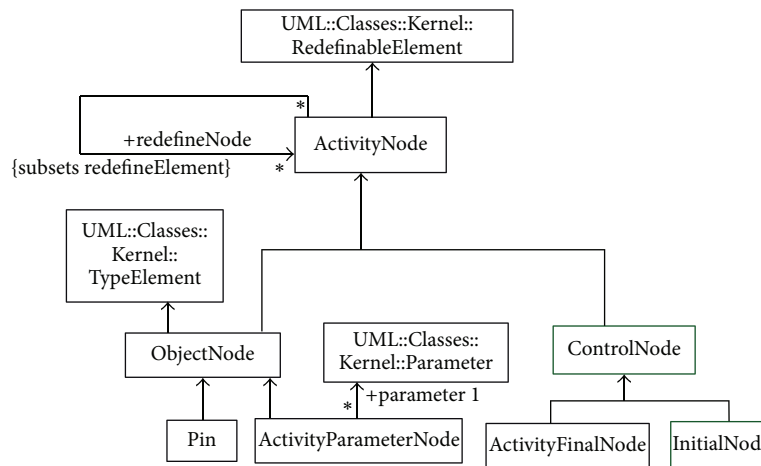
FIGURE 5: Metamodel of the OMG specification.
