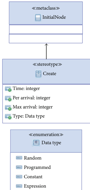
FIGURE 4: Relationship between metaclass and stereotype <<Create>>.
