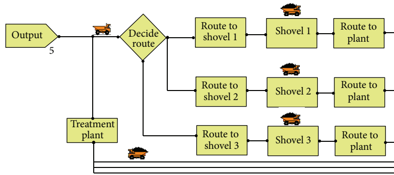
FIGURE 2: Limestone quarry simulation.
