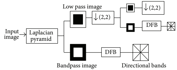
FIGURE 2: Contourlet Decomposition.
