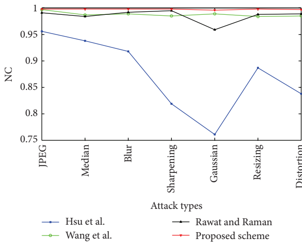
FIGURE 11: Comparison with existing zero-watermarking schemes.
