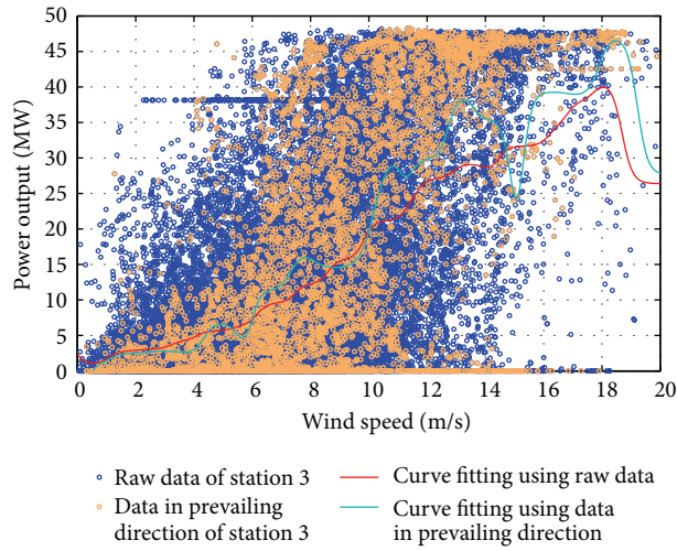
FIGURE 16: Curve fitting using the data in the prevailing direction of station 3.
