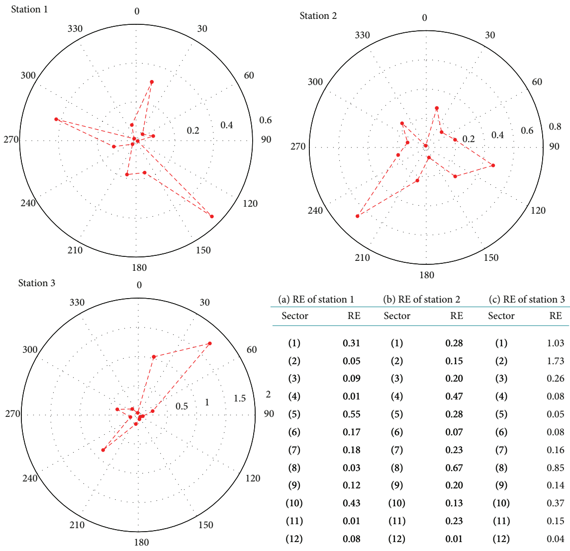
FIGURE 17: Performance of power curve modeling considering the wind direction.
