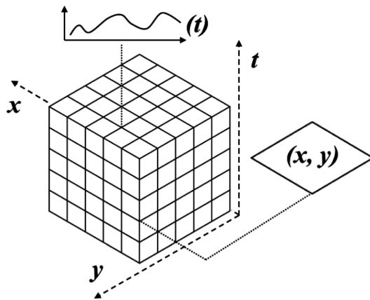
Figure 1. A three-dimensional data cube in which spatial data of two dimensions (e.g., latitude and longitude) are combined with a third dimension of time. In this view, a horizontal slice perpendicular to the time ( t ) axis corresponds to a geographic map while a line parallel to the time ( t ) axis represents a time series.
