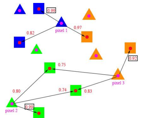
(a) Traditional connection in manifold alignment
