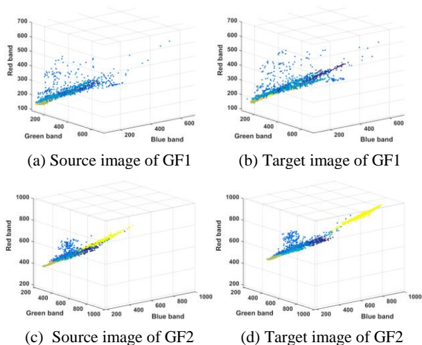
Fig.6 Scatter plots in original space (RGB bands) on 2 data sets.
