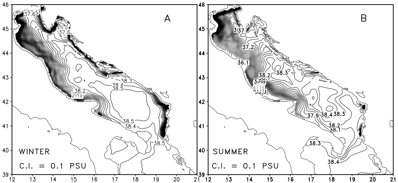
Fig. 7. Adriatic Intermediate Model (AIM). Seasonal surface salinity fields. (A): winter, (B): summer. Contour interval is 0.1 psu. Seasons definition as in Artegiani et al. (1997a, b).
