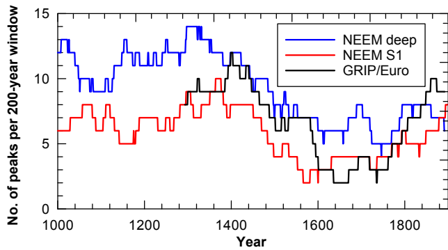
Figure 14. Fire peak frequency in a running 200-year window for the Eurocore at Summit (black), the NEEM deep core (blue), and the NEEM-2011-S1 core (red). Peaks detected in adjacent years were only counted as one.
