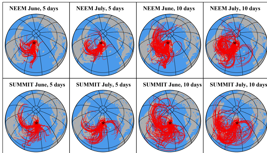
Figure 11. The 5- and 10-day backward air mass trajectories arriving at the NEEM and Summit sites in June and July 1978 (site arrival at 500 m above ground level).
