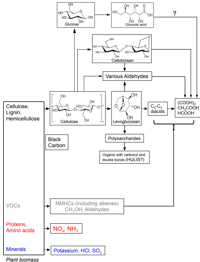
Figure 1. Proposed chemical pathways for formation of various chemical species identified in smoke aerosols. Adapted from Gao et al. (2003) and references therein, Kawamoto et al. (2003), and Abella et al. (2007).
