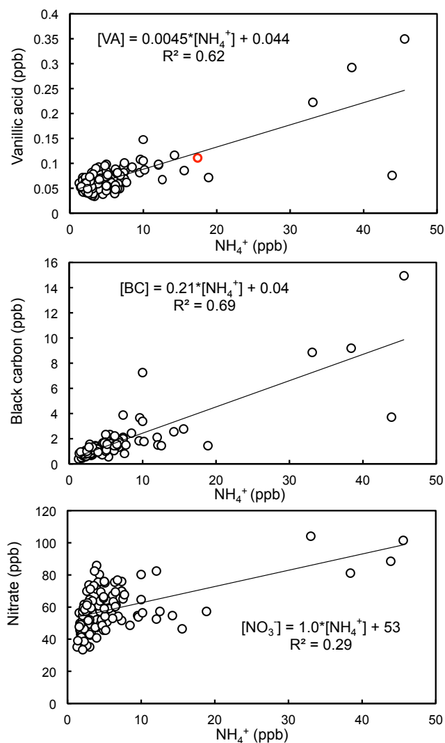
Figure 6. Annual mean concentrations of vanillic acid, BC, and nitrate vs. ammonium in snow layers deposited at D4 during pre-industrial times (from 1740 to 1870). For vanillic acid, we also report the point corresponding to the 1908 event (red circle).
