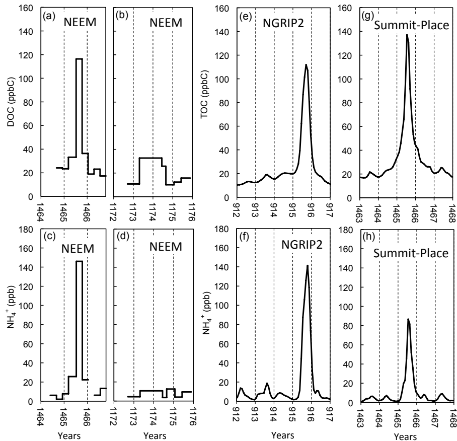
Figure 8. Example of OC changes along fire events in Greenland ice. Panels (a) to (d) are from the NEEM-2011-S1 ice core for which OC was measured with a UV oxidation method (Sect. 2) and ammonium on discrete samples analyzed with ion chromatography. Panels (e) to (h) are from North GRIP2 and Summit-Place (collected in 2015) ice for which ammonium was measured with a CFA system and OC was investigated with a CFA coupled to a total organic carbon analyzer (Sect. 2). The NEEM-2011-S1 and North GRIP2 cores were drilled with organic drilling fluid and the Summit-2015-Place core without.
