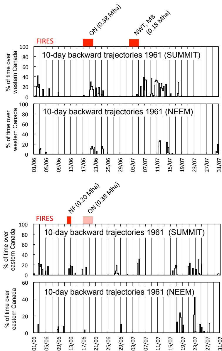
Figure 12. Fraction of time spent by air masses arriving at Summit and NEEM (10-day backward trajectories) at 500 m a.g.l. and having traveled over a forested area of western (top) and eastern (bottom) provinces of Canada during the severe fire conditions of June/July 1961 (Fig. 10). Some of the largest fires are indicated on top of the panels (red symbols) with corresponding burned area: Ontario and Northwest Territories in the West, Newfoundland and Labrador in the east. The Ontario fire was located in the western portion of the province and we report the red symbol on both panels. Area burned data are from the Canadian National Fire Database (Sect. 4.1).
