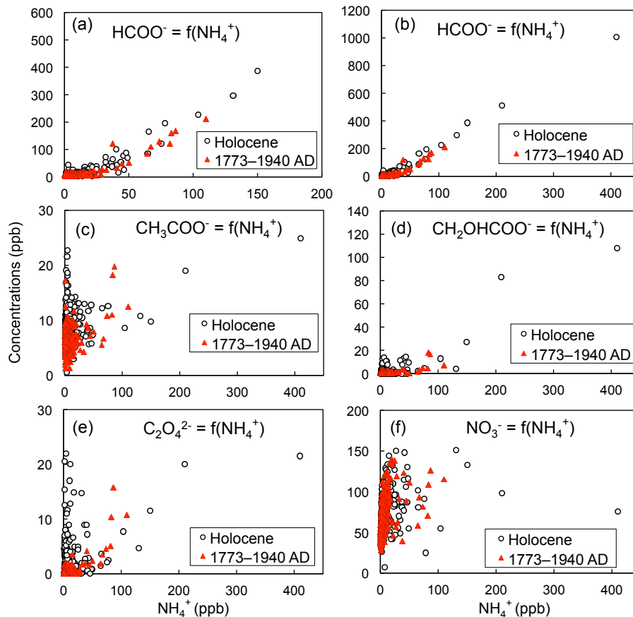
Figure 2. Concentrations of various carboxylates (a–e) and nitrate ( \text{NO}_3^- ), (f) as a function of ammonium ( \text{NH}_4^+ ) in Summit snow and ice layers. \text{HCOO}^- is formate, \text{CH}_3\text{COO}^- is acetate, \text{CH}_2\text{OHCOO}^- is glycolate, and \text{C}_2\text{O}_4^{2-} is oxalate. For formate, two panels (a and b) are shown to detail the relationship at ammonium concentrations lower than 200 ppb (a). The red triangles correspond to the layers deposited between 1773 and 1940 AD (520 values along the GRIP 93 firn core; Table 1); the black circles correspond to the Holocene period along the GRIP deep ice core (660 values between and 355 and 11 600 yr BP).
