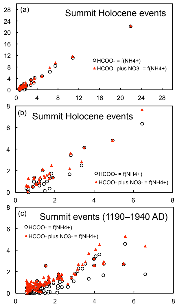
Figure 7. Ammonium vs. formate (formate plus nitrate) along \text{NH}_4^+ events at Summit. All concentrations are expressed in \mu\text{Eq L}^{-1} .
