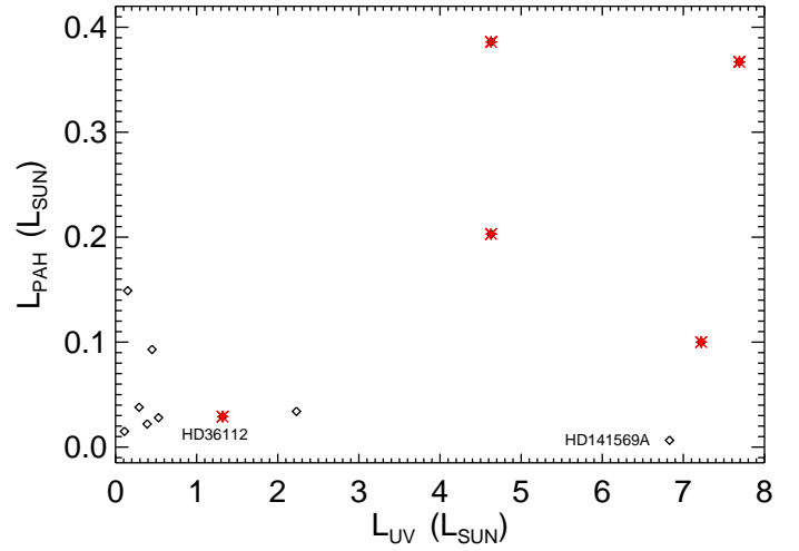
Fig. 6. L_{\text{PAH}} as a function of L_{\text{UV}} for the HAEBE sample. The red asterisks indicate sources where CO was detected in our spectra, the black diamonds the sources with non-detections.
