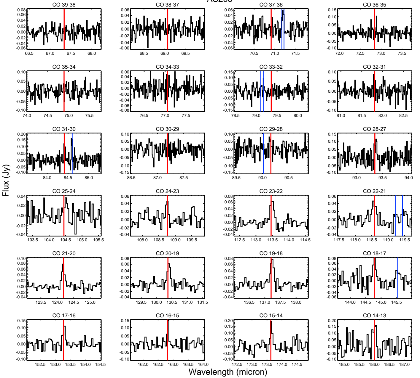
Fig. A.5. The spectra of AS 205, centered on the CO lines, indicated in red. The OH line at 84.42 \mu\text{m} blends with the CO J = 31 \rightarrow 30 line. In blue, we indicate the positions of other lines (CH + at 90 \mu\text{m} and [O I] at 145 \mu\text{m} ; rest are OH doublets).
