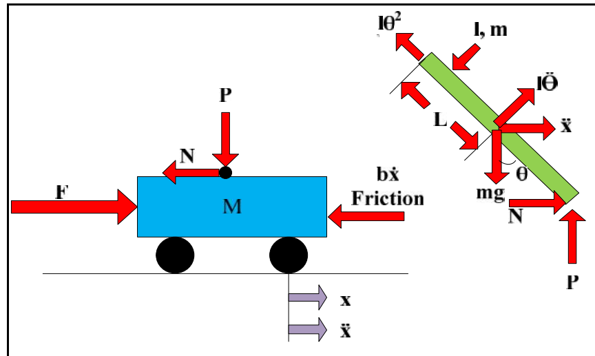
Figure 3.3: Free body diagram of the system
