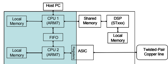
Figure 9. VDSL modem application
