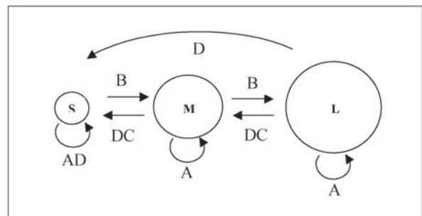
Fig. 2. Life cycle graph for the population of Arctophila fulva at the Liminka Bay. Arrows indicate transitions among patch size classes: (S) small, (M) medium and (L) large. Transitions between patch classes are: (A) survival in the same size class, (B) growth to a larger size class, (C) shrinkage to smaller size class and (D) production of a new patch.
