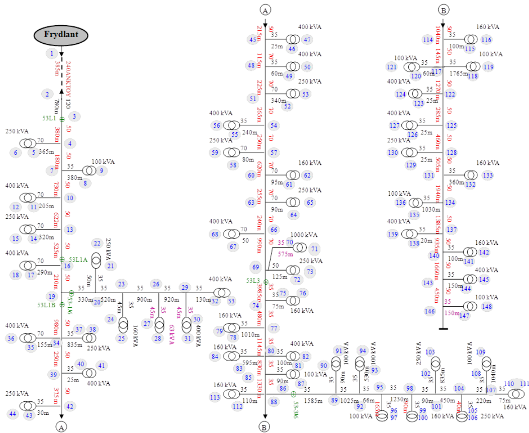
Fig. 1: The diagram of Frydlant network.
