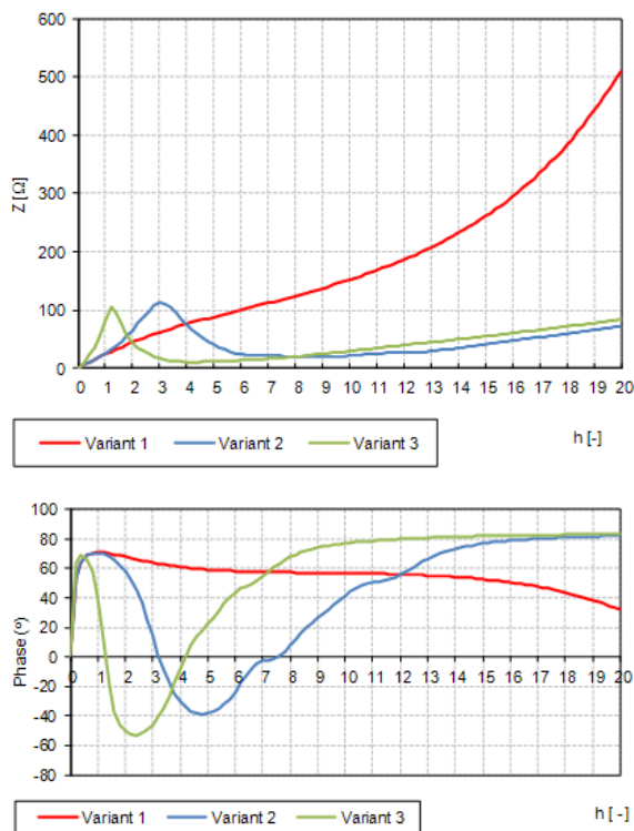
Fig. 7: The harmonic impedance and the phase shift of the network.
