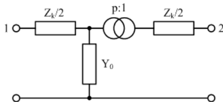
Fig. 2: Diagram of transformer.
