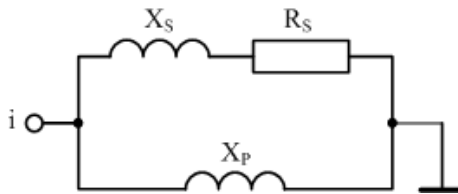
Fig. 4: Model according to CIGRE.
