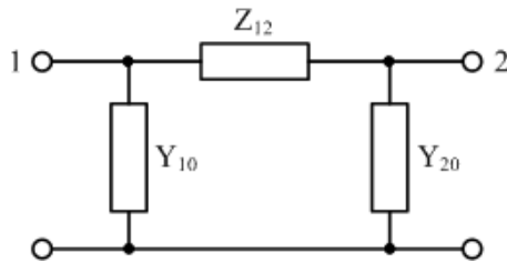
Fig. 3: Diagram of transmission lines.
