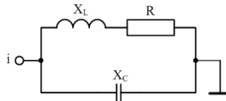
Fig. 5: Model with compensation.
