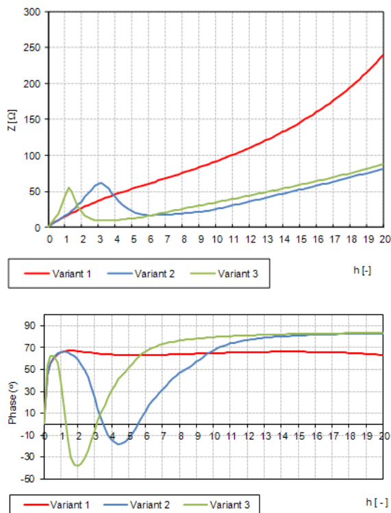
Fig. 6: The harmonic impedance and the phase shift of the network.
