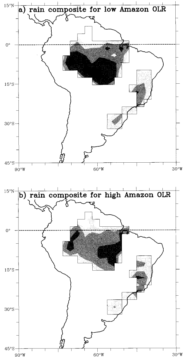
FIG. 14. As in Fig. 13 except that OLR is centered at 10^{\circ}\text{S} , 65^{\circ}\text{W} .
