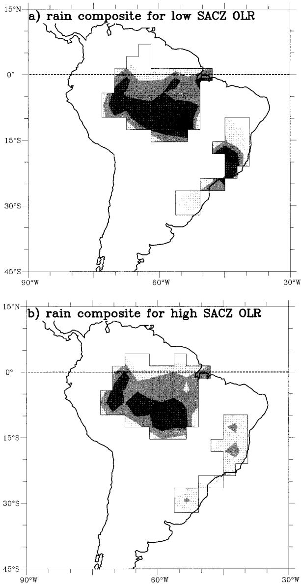
FIG. 13. Composite rainfall for periods when DJF OLR at 20^{\circ}\text{S} , 45^{\circ}\text{W} , filtered to include periods less than 30 days, is at least 1.5 standard deviations (a) below and (b) above mean. Data from stations within 2.5^{\circ} squares have been averaged. Shading starts at 3\text{ mm day}^{-1} with an interval of 3\text{ mm day}^{-1} . Thin lines depict regions where data are available.
