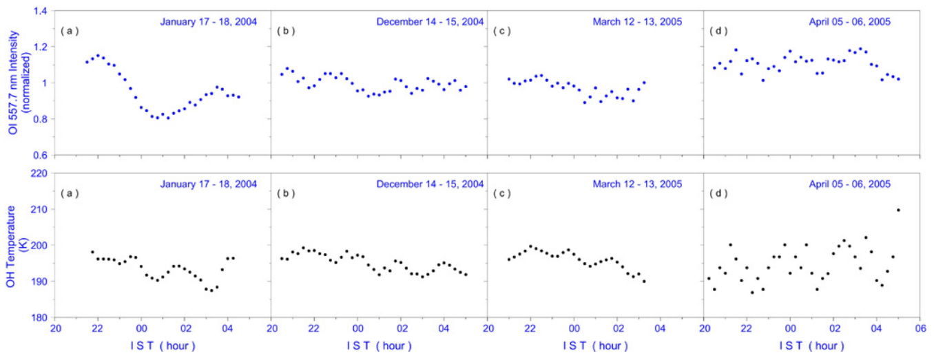
Fig. 4. Examples of gravity wave induced variations in OI 557.7 nm intensity (top row) and the OH temperature (bottom row).
