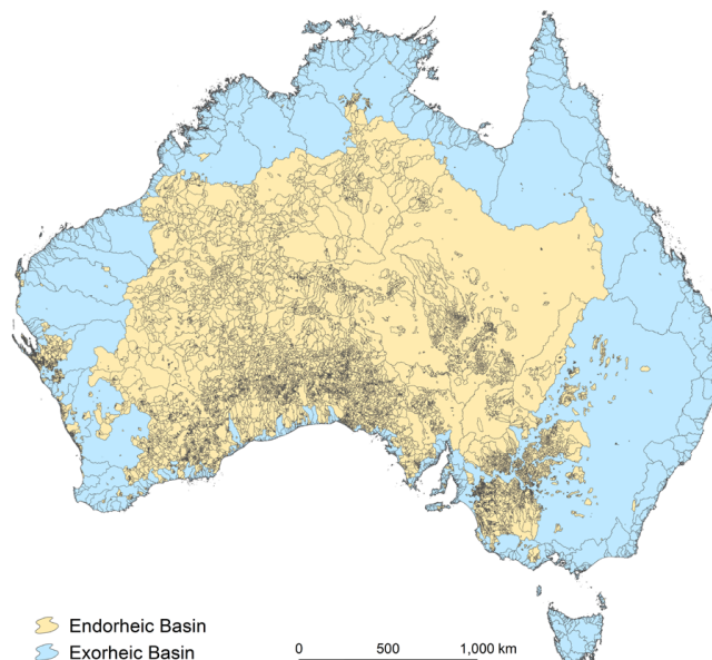
Figure 5. Drainage basins delineated from the 9 s DEM.
