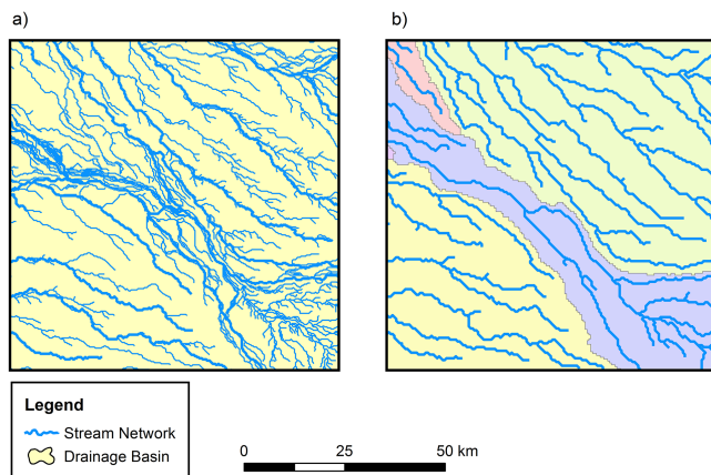
Figure 9. The stream network and drainage basins delineated by (a) this study and (b) supplied by the HydroSHEDS database for the area shown in the inset map of Fig. 4. By recognising distributary drainage connections, one drainage basin is delineated for these rivers draining into the Gulf of Carpentaria, while the HydroSHEDS database delineates multiple basins.
