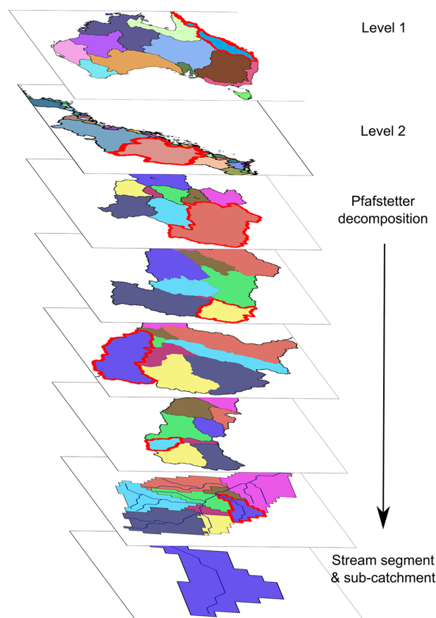
Figure 2. Components of the nested stream and catchment database. The nested hierarchy of catchments aggregates drainage basins at its highest levels and at its lower levels, sub-divides basins into successively smaller catchment units based on the Pfafstetter system. The smallest units in the catchment framework are the catchment areas draining to individual stream segments in the associated DEM stream network. Attributes describing the natural and anthropogenic environment of the stream and its catchment are contained in the related lookup tables. The area shown at each level is highlighted with a red boundary at the next higher level.
