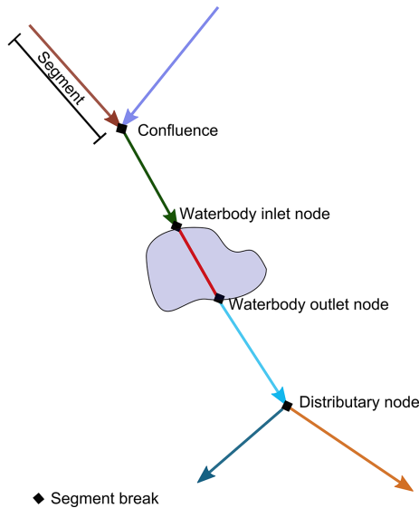
Figure 3. Breaks inserted into the DEM stream network at confluences, distributary nodes and water bodies. The breaks delineate uniquely identified stream segments.
