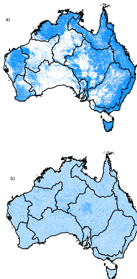
Figure 8. The stream network delineated by (a) this study and (b) that supplied by the HydroSHEDS database. Level 1 drainage divisions are indicated by the bold black lines.
