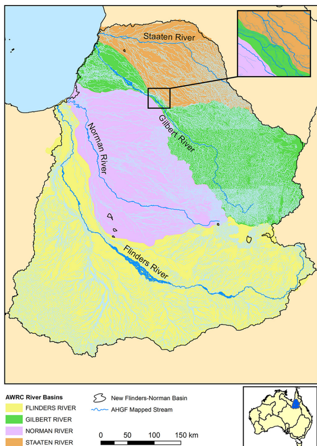
Figure 4. The Flinders–Norman Drainage Basin combining the catchment areas of the Norman, Flinders, Staaten and Gilbert rivers that are linked by floodplain distributaries. In contrast, the AWRC river basins delineate four separate river basins with boundaries drawn through the floodplain distributary channels. Note also the small areas of internal drainage.
