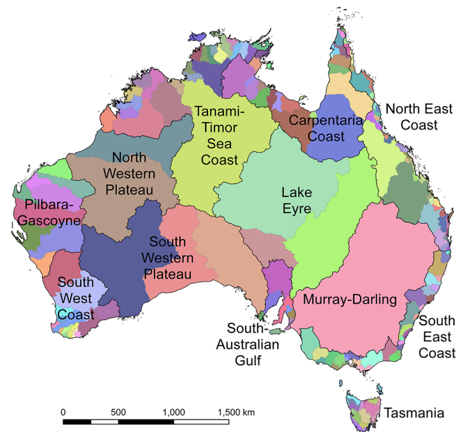
Figure 6. Levels 1 and 2 of the new hierarchically nested catchment framework. Shown are the Level 1 topographic drainage division names.
