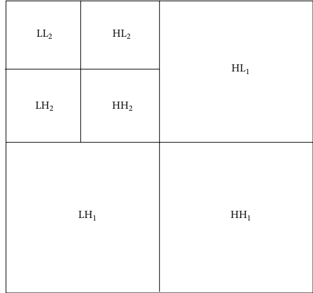
FIGURE 5: Two-level image decomposed using DWT for one color channel.
