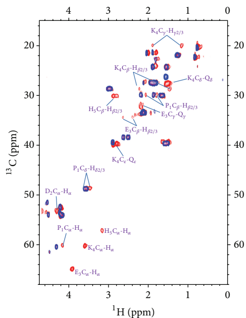
FIGURE 8: Selection of aliphatic regions in the ^{13}\text{C} - ^1\text{H} HSQC NMR spectra for PK9-H peptide, 2.5 mM, pH 10.5, and T 298 K, in the absence (blue) and in the presence (red) of 0.9 equivalents of Ni(II). New resonances due to Ni-binding have been labelled.
