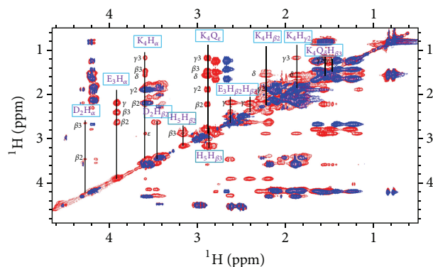
FIGURE 7: Selection of aliphatic region in the ^1H - ^1H TOCSY NMR spectra for PK9-H peptide, 2.5 mM, pH 10.5, and T 298 K in the absence (blue) and in the presence (red) of 0.9 equivalents of Ni(II). New resonances due to Ni-binding have been labelled.
