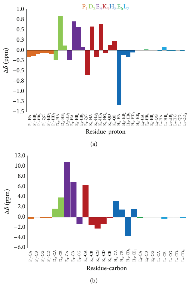
FIGURE 9: Plot of the observed ^1\text{H} proton (a) and ^{13}\text{C} carbon (b) chemical shift changes ( \Delta\delta = \delta_{\text{holo}} - \delta_{\text{apo}} ) for PK9-H peptide following nickel coordination.
