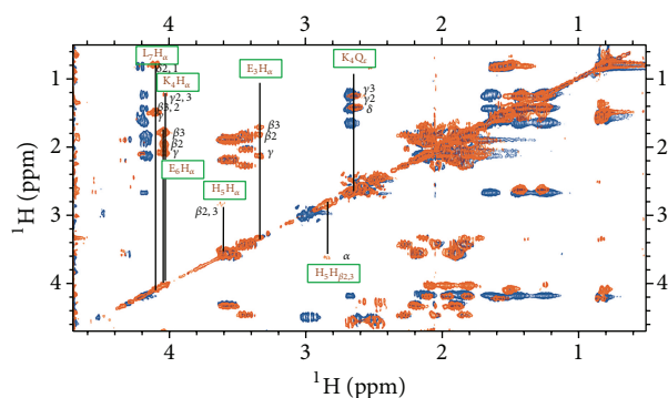
FIGURE 3: Selection of aliphatic region in the ^1\text{H} - ^1\text{H} TOCSY NMR spectra for PK9-H peptide, 2.5 mM, pH 11, and T 298 K in the absence (blue) and in the presence (orange) of 0.05 equivalents of Cu(II). New resonances due to Cu-binding have been labelled.
