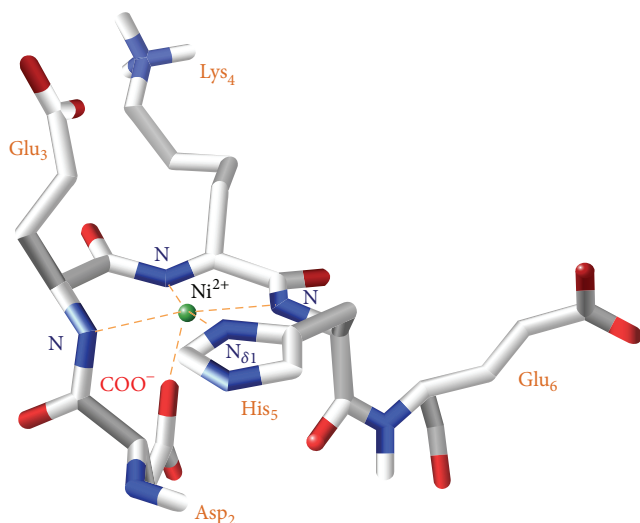
FIGURE 10: 3D structural model, derived from NMR structural constraints (ROEs), for the Ni(II) ion complexed with PK9-H peptide in a pentacoordinated geometry, with the involvement of the N\delta_1 imidazole nitrogen of the histidine residue, three deprotonated amidic nitrogens from the peptide backbone (belonging to His-5, Lys-4, and Glu-3 residues), and the carboxylate moiety from aspartyl (Asp-2) residue in the apical position, giving a \{N_{lm}, 3N^-, O^-\} species.
