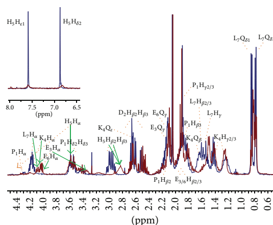
FIGURE 2: Superimposition of ^1\text{H} NMR spectra for the PK9-H peptide, 2.5 mM, pH 11, and T 298 K, in the absence (blue) and in the presence (red) of 0.05 equivalents of Cu(II). New resonances due to Cu-binding have been indicated by green arrows.
