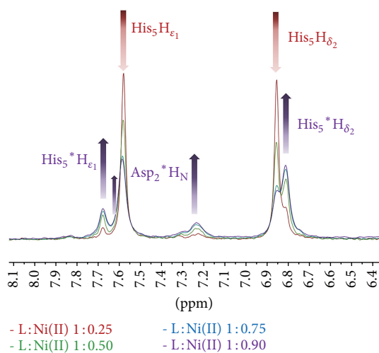
FIGURE 6: Superimposition of ^1H NMR spectra in the aromatic regions for the PK9-H peptide, 2.5 mM, pH 10.5, and T 298 K, with increasing amounts of Ni(II) from 1:0.25 to 1:0.90 metal to ligand molar ratios. New resonances due to Ni-binding have been labelled by asterisk*.
