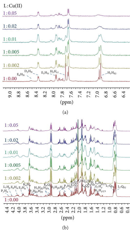
FIGURE 1: Stacked image of ^1\text{H} NMR spectra for the aromatic (a) and aliphatic (b) regions for the PK9-H peptide, 2.5 mM, and pH 7.6, T 298 K, with increasing amounts of Cu(II) from 1:0.00 to 1:0.05 metal to ligand molar ratios.
