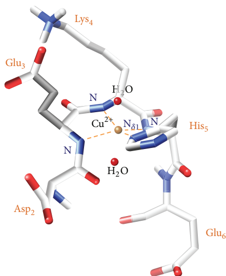
FIGURE 5: 3D structural model for the Cu(II) ion complexed with PK9-H peptide in a distorted tetragonal geometry, with the involvement of the N\delta_1 imidazole nitrogen of the histidine residue, and three deprotonated amidic nitrogens from the peptide backbone (belonging to His-5, Lys-4, and Glu-3 residues), giving a \{N_{lm}, 3N^-\} species.
