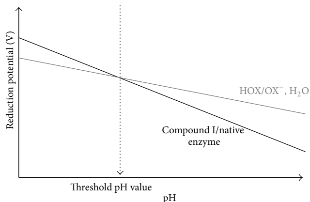
FIGURE 3: Illustration (according to [17]) of the pH threshold value above which the oxidation of the halogen by mammalian heme peroxidase will be thermodynamically unfavorable. The reduction potential of the couple Compound I/native enzyme and the couple halogen ( \text{X} = \text{chloride, bromide} ) \text{HOX}/\text{OX}^- is expressed with an illustrative function of the pH, at a specific concentration of enzyme and substrates.
