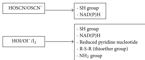
FIGURE 5: Target group of hypothyocyanite, hypiodite, and iodine. Due to its low oxidation power, hypothyocyanite is relatively specific and is not reactive against all thiols. In vivo , hypiodite seems to be selectively directed against reduced pyridine nucleotide because even the presence of excess glutathione and methionine does not thoroughly inhibit their oxidation. HOSCN/OSCN - : acidic or basic form of hypothyocyanite; HOI/OI - : acidic or basic form of hypiodite; and I 2 : iodine.
