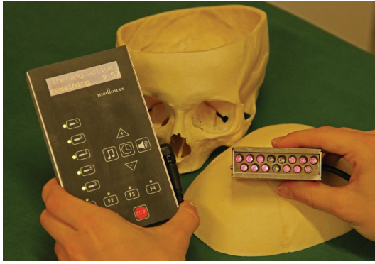
FIGURE 3: The medlouxx system including the LED applicator.
