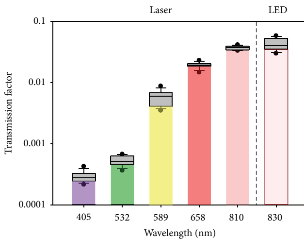
FIGURE 4: Transmission factor of different types of laser (modified from [20]) and of the new medlouxx system (LED). The results from violet (405 nm), green (532 nm), yellow (589 nm), red (658 nm), and infrared (810 nm) lasers are based on a previous study [20]. The system based on LED showed the highest mean value of the transmission factor (830 nm infrared light). The lines in the boxes represent the median, the ends of the boxes define the 25th and 75th percentile, and the error bars define the 10th and 90th percentile.
