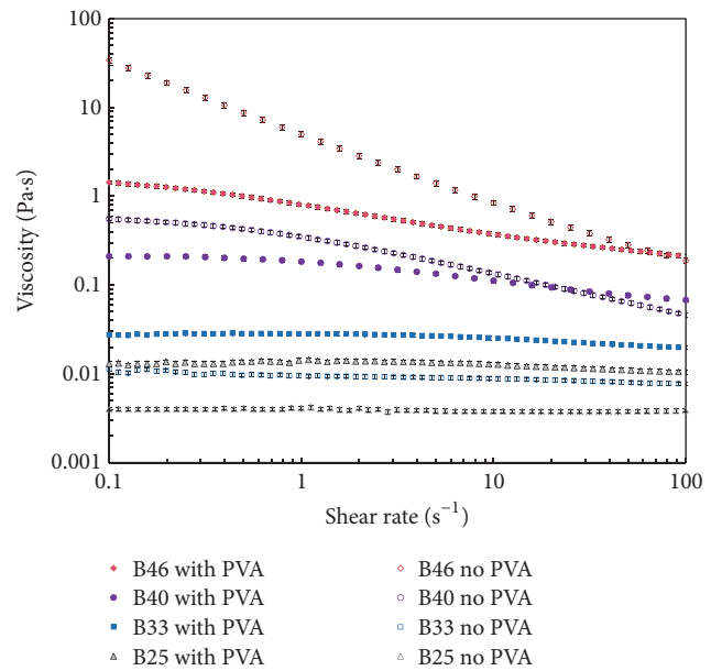
FIGURE 6: Viscosity versus shear rate for slurries containing 25 to 46 vol% of alumina particulates. Slurries with and without PVA. PVA content of 6% of weight of particulates for slurries containing PVA.
