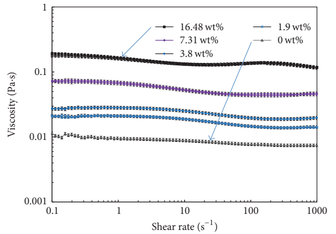
FIGURE 5: Viscosity versus shear rate for back-forward loop for B33 slurries with varied PVA content from 0 to 16.48 wt%.
