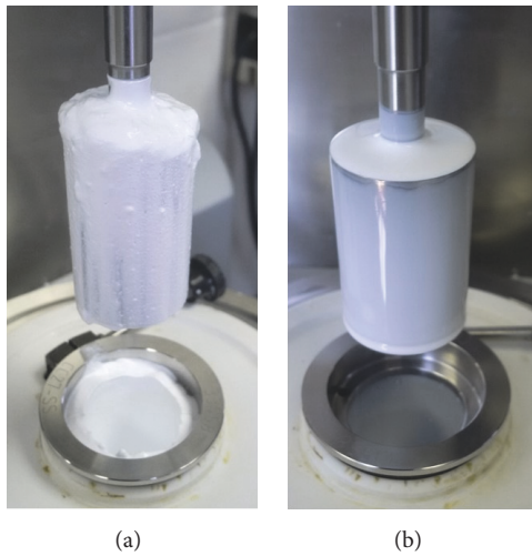
FIGURE 4: Foaming structure for B33 slurries with low acid content of 0 and 0.01 wt% (a) and liquid-like B33 slurries with acid content higher than 0.04 wt% (b).
