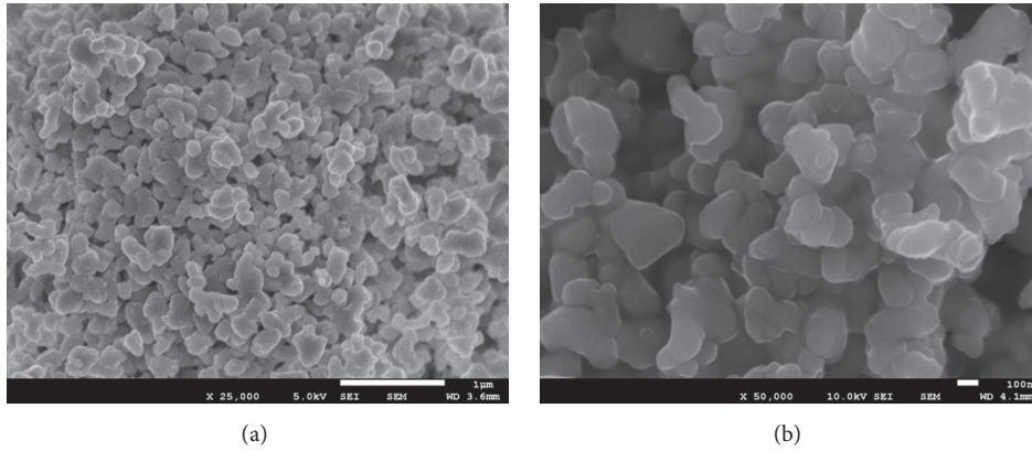
FIGURE 1: FEG-SEM micrographs of alumina particulates. Scale 1 micron (a) and 100 nm (b).
