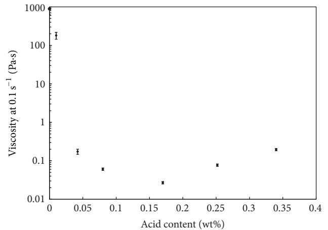
FIGURE 3: Viscosity at 0.1 \text{ s}^{-1} shear rate versus acid content for B33 slurries with varied acid content from 0 to 0.34 wt%.
