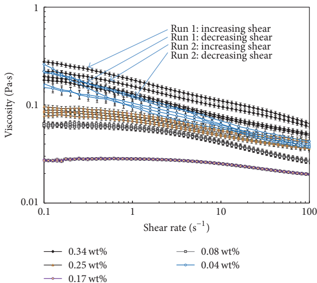
FIGURE 2: Viscosity versus shear rate for two consecutive back-forward loops for B33 slurries with varied acid content from 0.04 to 0.34 wt%.
