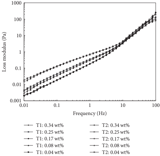
FIGURE 7: Loss modulus versus frequency for B33 slurries containing varied acid content from 0.04 to 0.34 wt%. Two tests illustrated T1 and T2.
