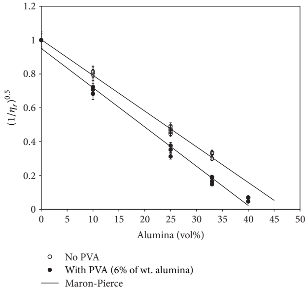
FIGURE 10: Relative viscosity versus alumina concentration for slurries with and without PVA containing 0 to 40 vol% of alumina particulates. Modeling using Maron and Pierce equation.
