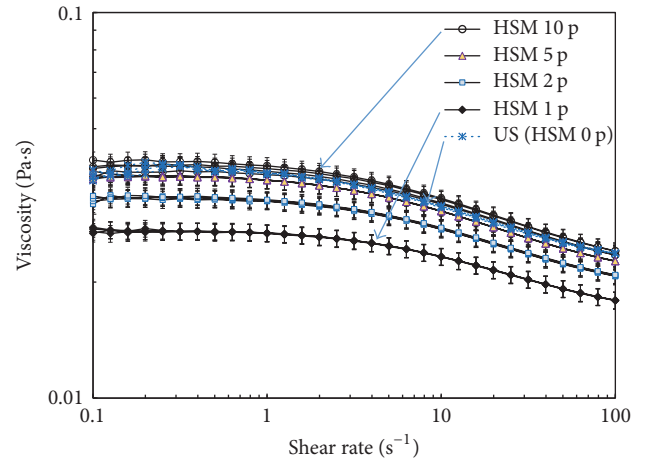
FIGURE 9: Viscosity versus shear rate for B33 base slurry (0.17 wt% acid and 3.80 wt% PVA) preparation using HSM. Consecutive pass in HSM using the same mixture from 1 pass to 10 passes. Slurry with 0 passes corresponds to US.
