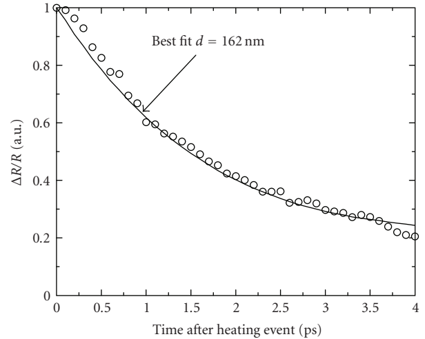
FIGURE 7: TTM using k_p fit to TTR experimental data taken on a 2\mu\text{m} Au nanoporous film with ligament thicknesses around 100 nm. The fit was achieved by iterating d , the ligament, or “nanowire” thickness. A best fit was achieved with a thermal conductivity calculated using d = 162\text{ nm} , in relatively good agreement with the ligament thickness of the nanoporous Au film that was tested.
