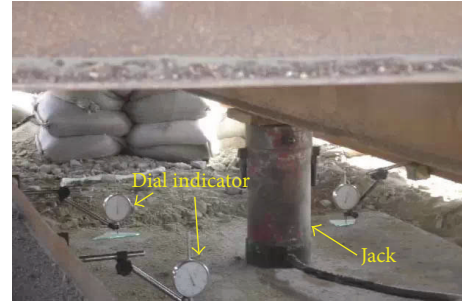
FIGURE 6: Field diagram of shallow flat plate static load test.
