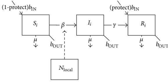
FIGURE 2: Schematic diagram of the basic SIR model with preexisting immunity.
