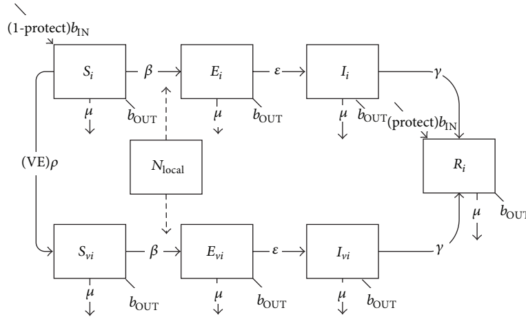
FIGURE 11: Schematic diagram of varicella transmission and vaccination.
