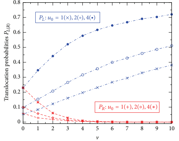
FIGURE 3: Translocation probabilities P_L (blue dash-dotted lines) and P_R (red dashed lines) are plotted against v for the channels with different effective potentials u_0 : 1( \times and + ), 2( \circ and \diamond ), and 4( \bullet and * ). Other parameters and symbols are the same as in Figure 2.
