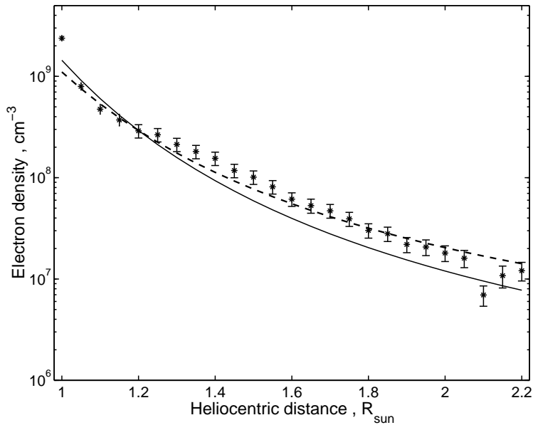
Fig. 10.— Comparison of the present modeled density distribution (asterisks with error bars) with hydrostatic density model at T_{\text{sh}} = 1.43 \text{ MK} (solid line) and T_{\text{sh}} = 1.72 \text{ MK} (dashed line).
