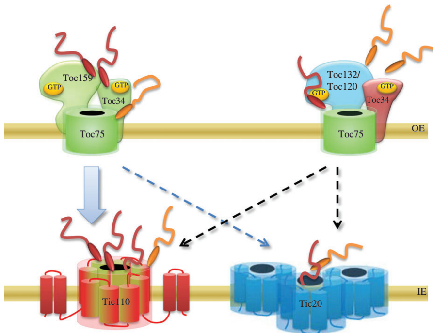
Figure 2 Hypothetical model of two distinct TOC core complexes and two independent channels at the TIC translocon.
