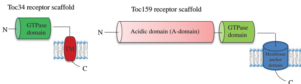
Figure 1 General scheme of the molecular scaffold of Toc34 and Toc159 receptor families.
