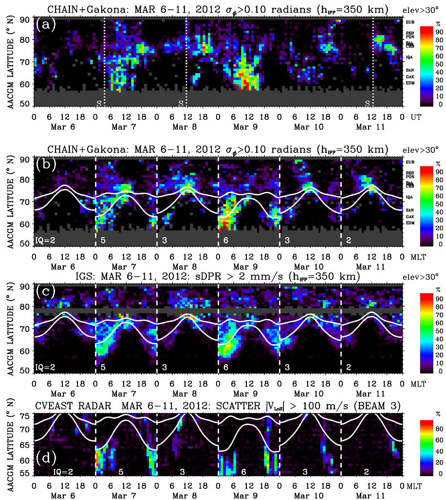
Figure 3. The occurrence of phase scintillation ( a, b ) \sigma_{\phi} > 0.1 rad, ( c ) sDPR > 2 \text{ mm s}^{-1} , and ( d ) Christmas Valley East radar backscatter ( V_{LOS} > 100 \text{ m s}^{-1} ) from 6 to 11 March. The maps are shown as a function of AACGM latitude and ( a ) UT or ( b–d ) MLT. The dotted vertical lines in the top panel indicate interplanetary shock arrival times in UT. The dashed vertical lines separate days mapped in MLT. The IQ value of the statistical auroral oval is chosen approximately proportional to a maximum 3-hourly Kp index.
