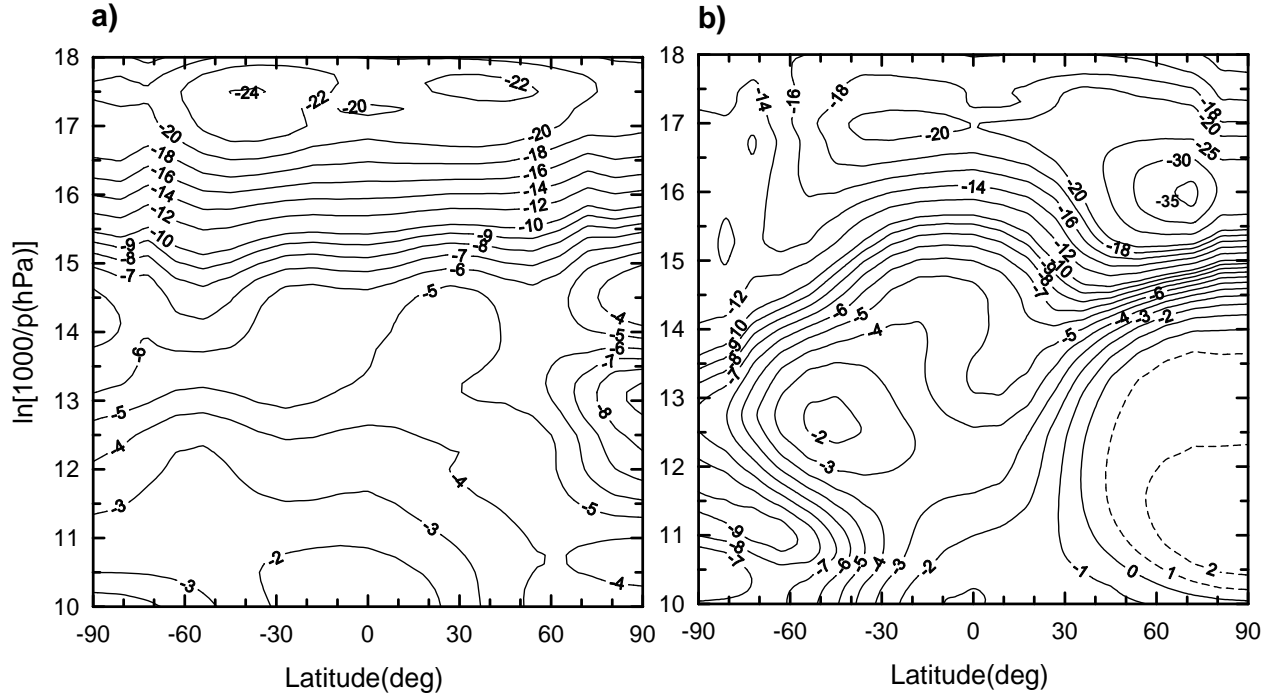
Fig. 9. Latitude-height distributions of heat influx in the CO 2 15- \mu m band in K/day in the UMLT region for 16 March (a) and 1 July (b), based on vertical profiles of temperature from the MSISE-90 model (Hedin, 1991). The dashed isolines correspond to atmospheric heating.
