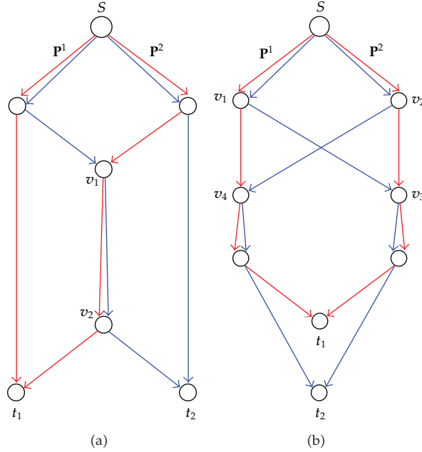
Figure 3: (a) A simple multicast network with two terminals has only one encoding node; (b) A feasible multicast network with two terminals has two encoding nodes. But it is not a simple multicast network, because if we delete (v_1, v_3) and (v_2, v_4) , this multicast network is also feasible.
