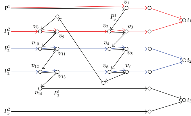
Figure 5: A simple cyclic multicast network in which paths P_3^1 and P_2^1 have common nodes.
