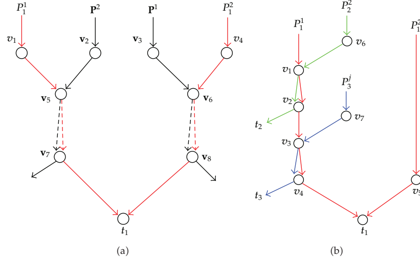
Figure 4: (a) One subnetwork of a feasible acyclic multicast network, in which if we blot out the red color, two encoding nodes v_5 and v_6 disappear. Here, at least one color path passes through the bold black links; (b) The other subnetwork in which if we blot out red color, two encoding nodes v_1 and v_3 disappear.
