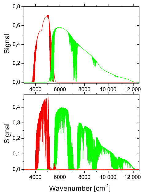
Figure 5. Lamp spectrum (top) and solar spectrum (bottom) recorded with the dual-channel prototype. The primary detector covers the spectral section observed with the standard EM27/SUN; the secondary detector covers the 4000–5500 \text{cm}^{-1} region.
