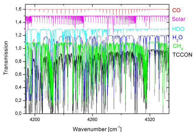
Figure 6. Spectrum simulated for TCCON resolution showing the relevant absorption features in the spectral region under consideration.
