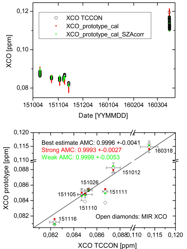
Figure 11. XCO deduced from the dual-channel prototype and the TCCON site Karlsruhe. Upper panel: time series of XCO. Lower panel: XCO values measured with the prototype as a function of the collocated TCCON XCO values (AMC denotes air mass correction). The error bars are the standard deviations of the intraday scatter. In the upper panel, all available TCCON values have been taken into account, whereas for the calculation of the statistics shown in the lower panel the TCCON measurements have been restricted to the observing hours of the prototype, because the intraday variability is not negligible in the case of XCO. As indicated by the calibration factors, the choice of the air mass correction does not critically impact the level of agreement found between the prototype and the TCCON XCO observations. The lower panel of the figure in addition shows XCO results derived from high-resolution mid-infrared spectra (open diamonds), analysed as described by Kiel et al. (2016b) (the calibration factor of 0.954 recommended by Kiel et al. has been applied to the mid-infrared data to match with the calibration of the TCCON).
