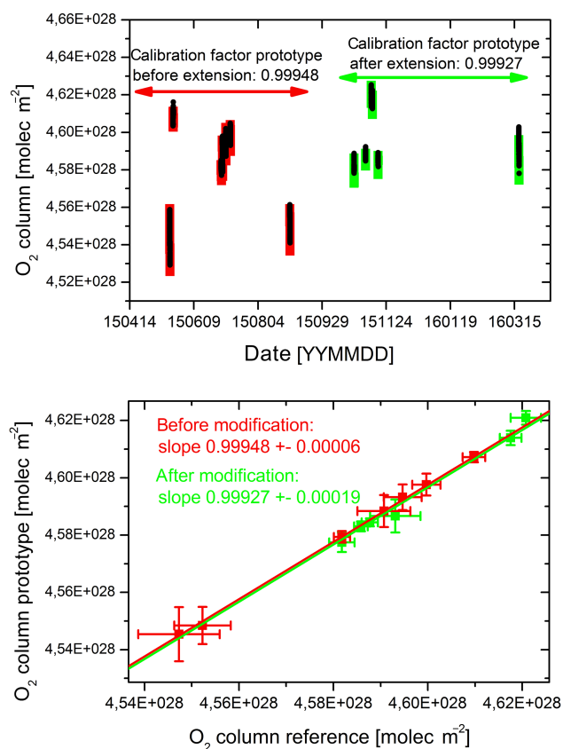
Figure 8. Total column amounts of molecular oxygen measured with the EM27/SUN used as a reference (data in black) and the prototype before and after the implementation (before: red; after: green) of the secondary channel. The implemented extension did not affect the characteristics of the prototype. Upper panel: time series of the O_2 column amounts as recorded with the reference spectrometer and the prototype. Lower panel: Mean daily O_2 column amounts as recorded with the prototype as a function of the values recorded with the reference spectrometer. The error bars shown are the standard deviation of the intraday scatter. The calibration factors before and after the modification of the prototype are in mutual agreement.
