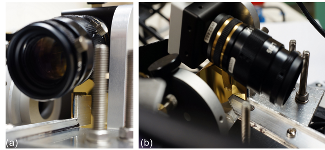
Figure 2. Close-up of the plane mirror used for decoupling of the secondary beam. (a) (left side) shows the support arm which carries the mirror. The mirror itself is seen from the back. On the left, parts of the circular mounting of the adjustable iris are seen. Behind the contours of the plane mirror, the larger off-axis paraboloid is located. Above the mirror, the camera used for the camera-controlled solar tracker is located. (b) (right side) offers a different perspective: below the camera, the front side of the plane mirror is seen. The frame of the iris is seen from the back.
