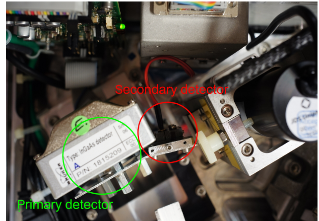
Figure 4. This image provides a top view of the detector units. The primary detector remains in its standard detector box; the supporting structure for the secondary field stop is mounted on the box of the primary detector. The secondary detector and the Ge filter are accommodated in a separate holder, which can be adjusted laterally with respect to the field stop.
