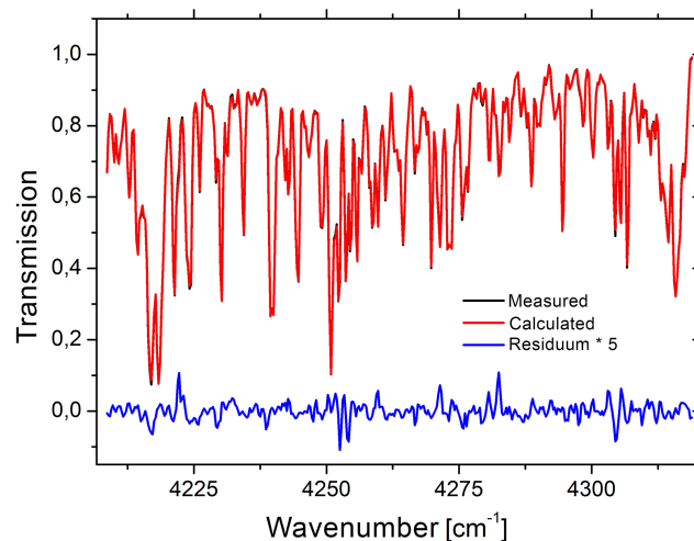
Figure 7. Typical spectral fit for the selected CO fitting region ( 4210\text{--}4320\text{ cm}^{-1} ). Interfering species are \text{CH}_4 , \text{H}_2\text{O} , and HDO.
