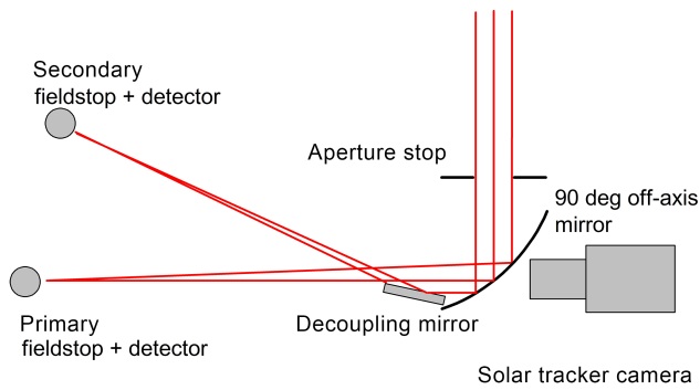
Figure 1. Schematic drawing of the detector branch of the extended EM27/SUN. The camera is located above the drawing plane and images the primary field stop. For clarity, the camera position has been shifted to the right in the drawing; it actually is located above the off-axis mirror.
