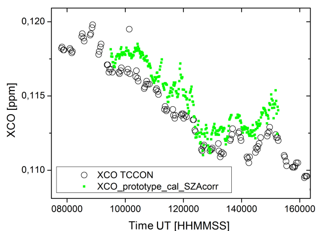
Figure 12. XCO intraday variability as observed during 18 March 2016, by the TCCON spectrometer and the dual-channel prototype.
