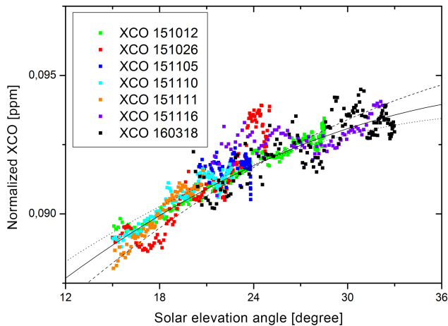
Figure 10. Apparent air mass dependency of the XCO data observed with the dual-channel prototype. For the air mass correction, we applied a second-order polynomial fit, choosing 25^\circ as the neutral point. For establishing the correction, spectra taken between 15^\circ and 33^\circ SEA have been taken into account. This choice results in the functional form (1 + 0.0027 \times (\text{SEA} - 25^\circ) - 0.00007 \times (\text{SEA} - 25^\circ)^2) , wherein SEA denotes the solar elevation angle (solid curve). For estimating the uncertainty introduced by the air mass correction when comparing the prototype XCO results with the TCCON, the linear term of the fit has been increased to 0.0034 (overcorrection, dashed curve) and decreased to 0.0022 (undercorrection, dotted curve).
