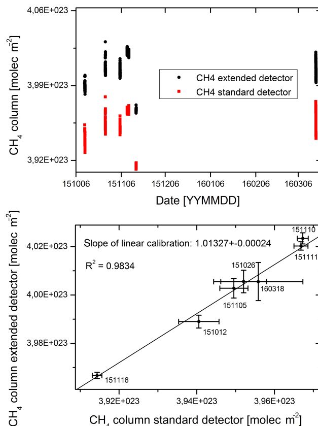
Figure 9. Comparison of methane column amounts as derived from the primary and secondary spectral channel. Upper panel: time series of methane columns. Lower panel: daily mean values of methane columns derived from the extended detector as a function of the methane columns derived from the standard detector. The error bars are the standard deviations of the intraday scatter. A linear fit of the calibration factor suggests a systematic spectroscopic offset of 1.013. There is no indication of a drift of the instrumental characteristics of the extended detector results with respect to the standard detector.
