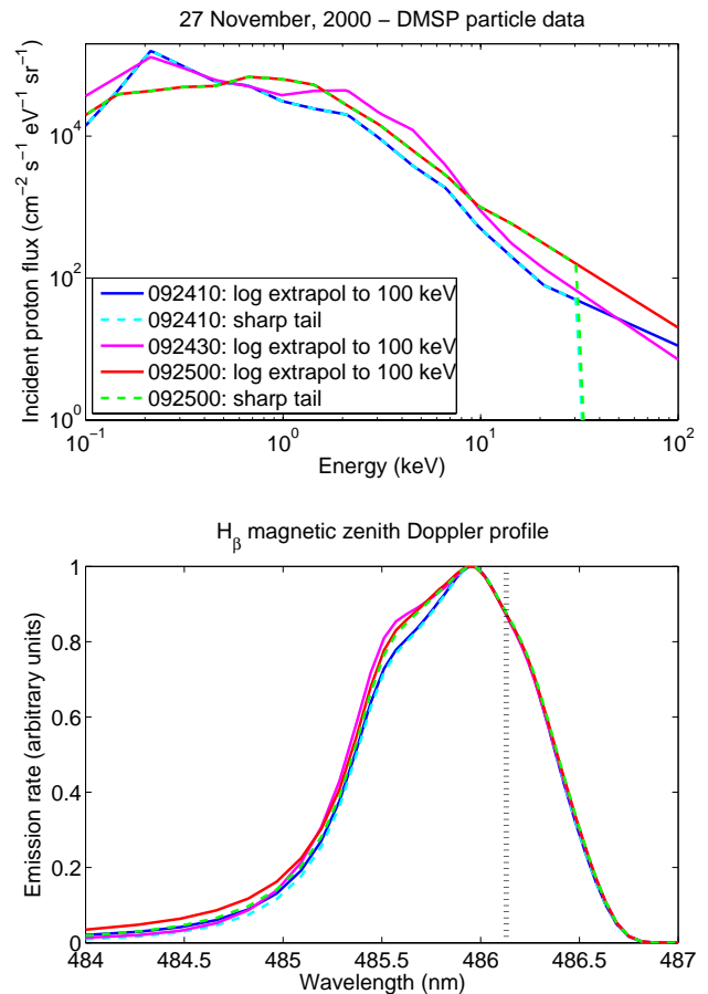
Fig. 12. (top) DMSP F12 input ion fluxes with and without high energy extrapolation. (bottom) Doppler-shifted H_{\beta} profiles along the magnetic zenith resulting from the H^+/\text{H} model driven by the DMSP input spectra above.
