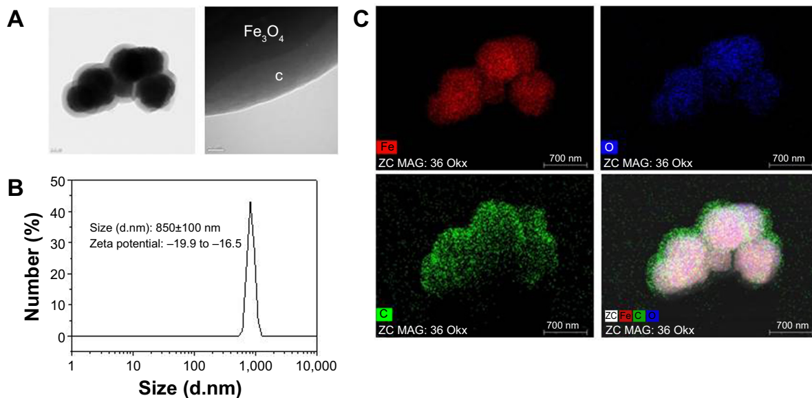
Figure 1 Morphology and size distribution of Fe 3 O 4 @C.
