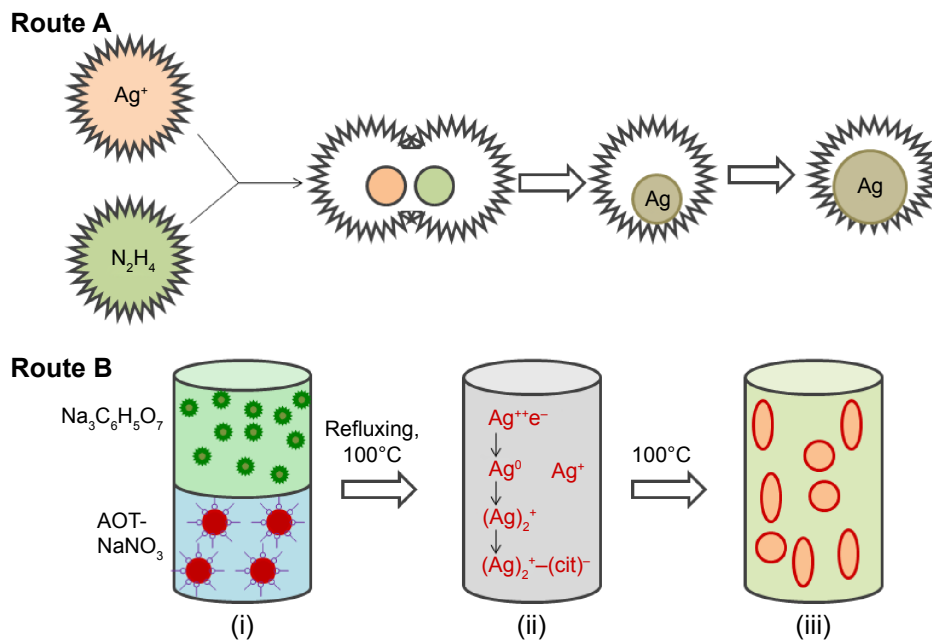
Figure S1 Schematic representation of synthesis of Ag nanoparticles and nanorods.
