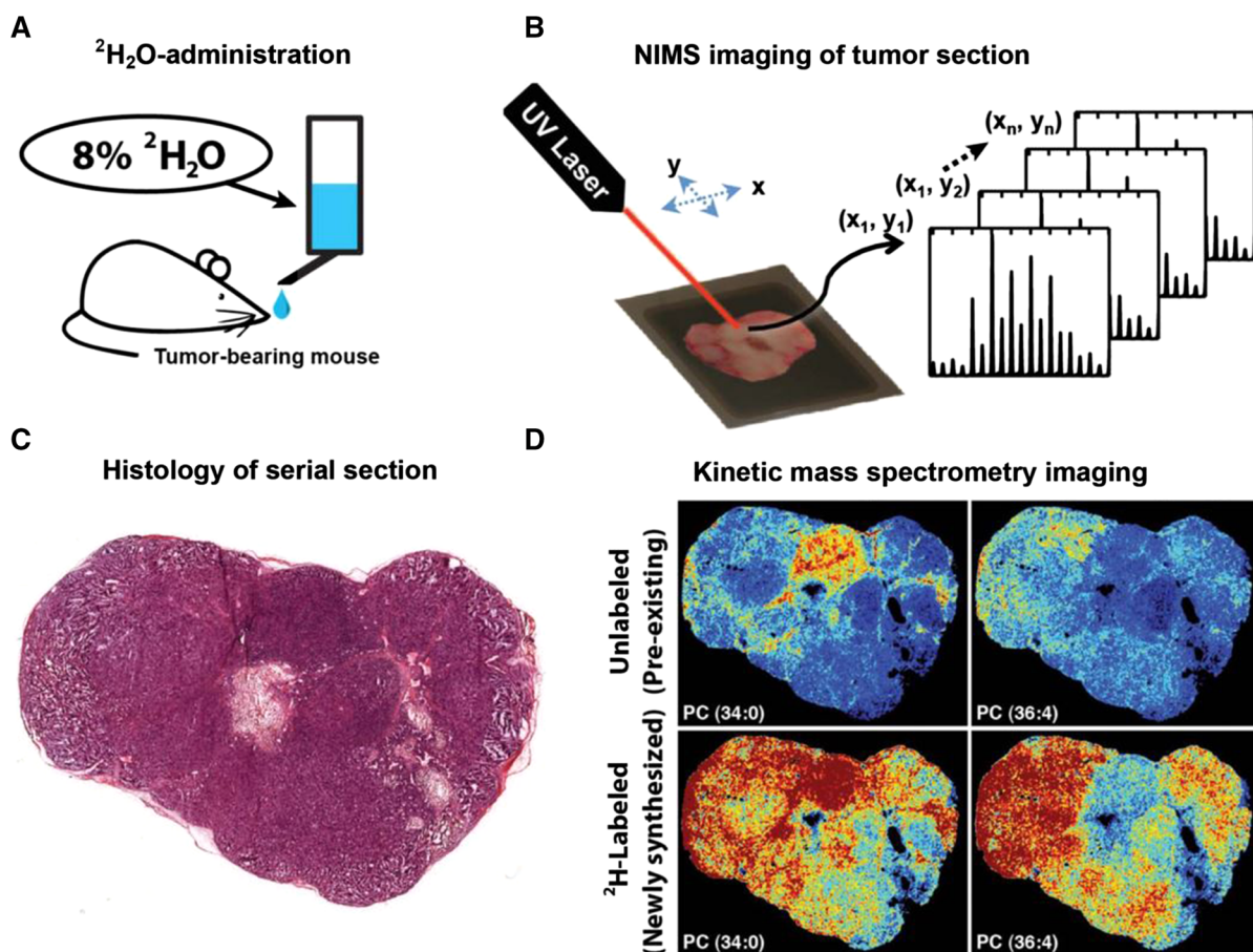
Fig. 8 Example of kinetic mass spectrometry imaging—experimental workflow for using kMSI to define spatial heterogeneity of lipid composition and biosynthesis. A A tumor-bearing mouse is administered ^2\text{H}_2\text{O} -enriched water to incorporate deuterium into tissue as a result of active metabolism. B The deuterium-enriched tumor is excised, sectioned and imaged using NIMS. An individual mass spectrum is generated for each pixel every 50 \mu\text{m} , with spectra comprised of isotopologues from both ^2\text{H} -
