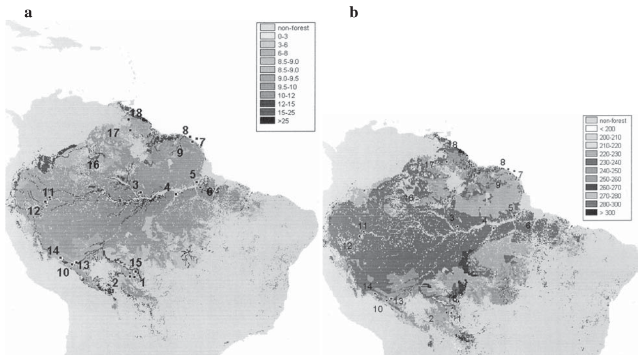
Fig. 2. Variation of soil properties across Amazonia. Data derived from the IGBP Global Soil Data Task (2000). a. Total carbon content (kg.m -2 ) in the top 1 m. 1 kg.m -2 = 10 t.ha -1 . b. Total available water capacity in the top 1 m (mm). In many Amazonia regions soils data are very sparse and these maps are only approximate. Plot numbers as in Fig. 1.
