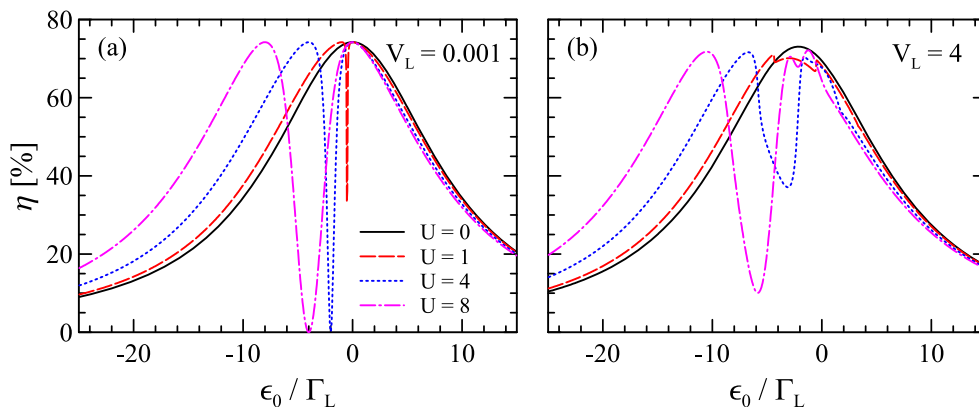
Fig. 3 Efficiency \eta as a function of the quantum dot level \epsilon_0 for a small eV_L/\Gamma_L = 0.001 and b large eV_L/\Gamma_L = 4 . The other parameters are the same as in Fig. 2
