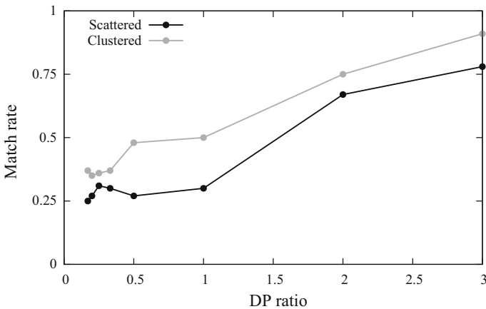
Fig. 10 Impact of the DP ratio on the match rate
