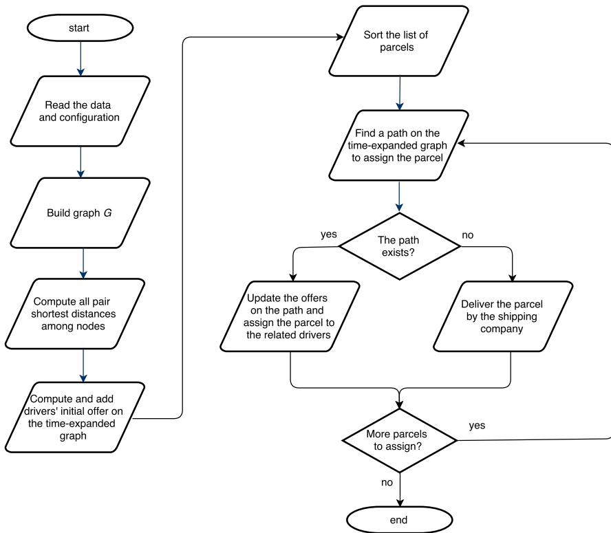
Fig. 4 Flowchart of the time expanded graph based heuristic
