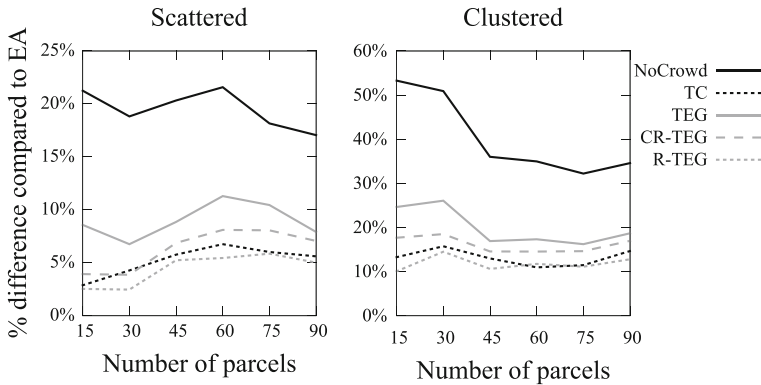
Fig. 11 Impact of the number of parcels, compared to the exact solutions
