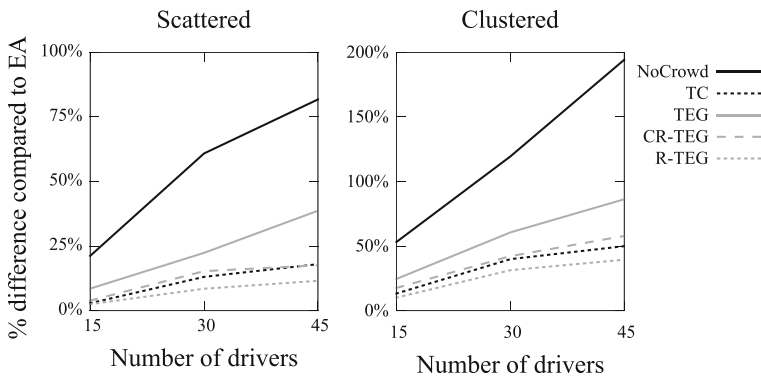
Fig. 12 Impact of the number of drivers, compared to the exact solutions
