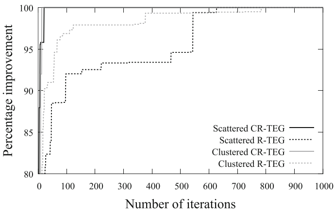
Fig. 14 Convergence speed of the CR-TEG and R-TEG heuristics
