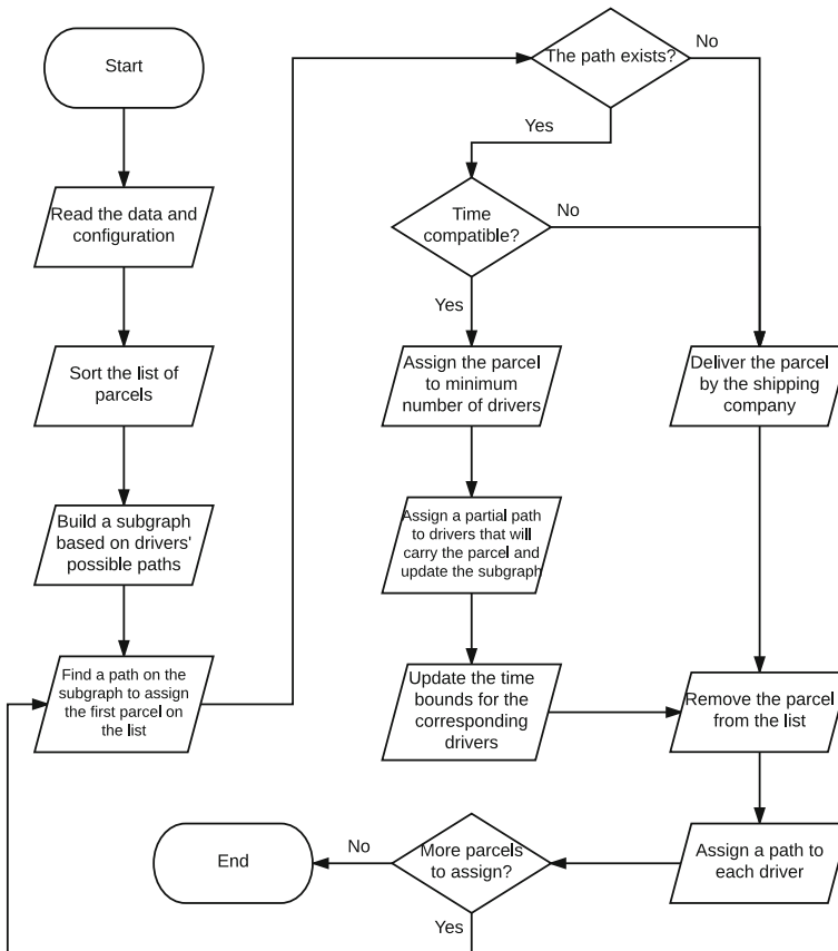
Fig. 2 Flowchart of the TC-heuristic
