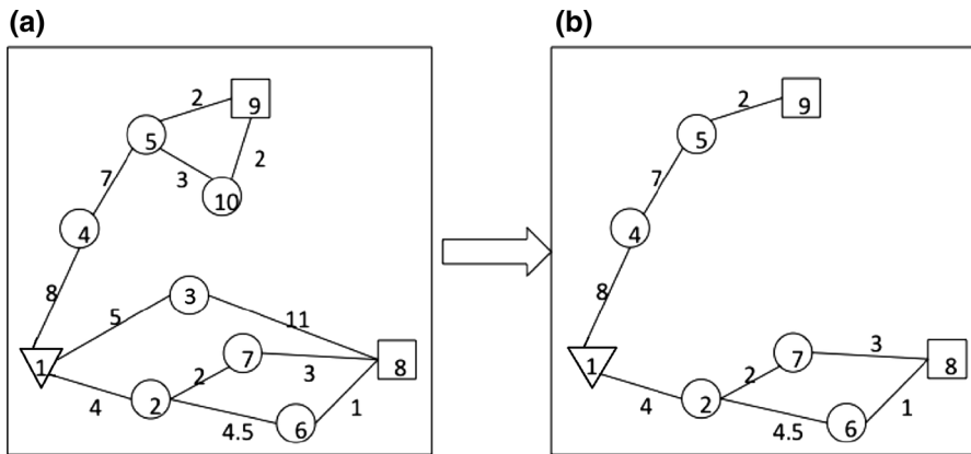
Fig. 1 An example of building a subgraph a The original graph b The subgraph
