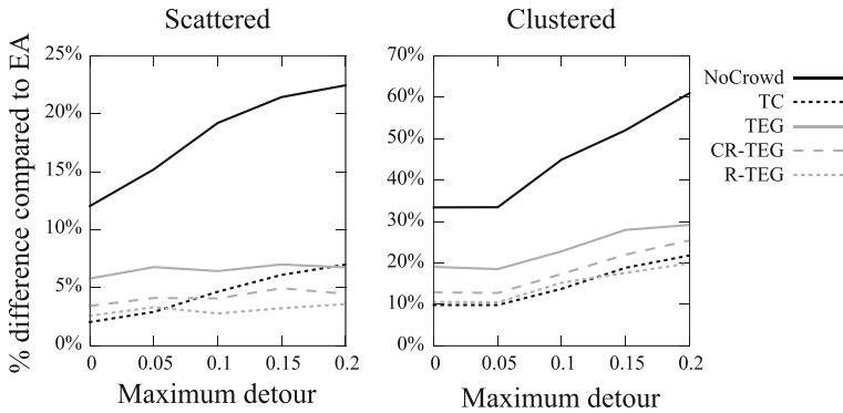
Fig. 13 Impact of \delta , compared to the exact solutions
