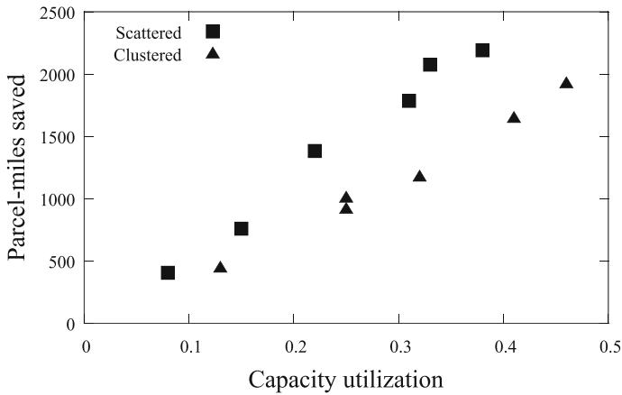
Fig. 9 Impact of driver's capacity utilization on parcel-miles saved
