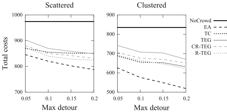
Fig. 7 The impact of maximum detour on total cost (#driver = 15, #parcel = 30)
