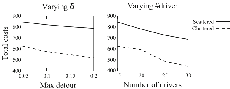
Fig. 8 The comparison of varying \delta given #driver = 15, and varying #driver given \delta = 0.05
